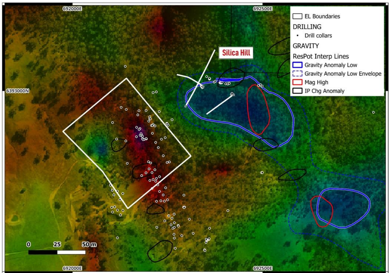
Figure 2: Plan view of the Silica Hill prospect showing the proposed downhole electromagnetic (DHEM) transmitter loop (white polygon) and selected Phase 2 drill hole traces (white lines), overlaid on gravity imagery with interpreted gravity, magnetic and IP anomalies. Silica Hill is associated with a prominent gravity low, with known mineralisation occurring along the gravity gradient at its western margin. The planned DHEM survey will investigate potential off-hole conductors and extensions of sulphide mineralisation at depth, beyond the existing drill coverage.
