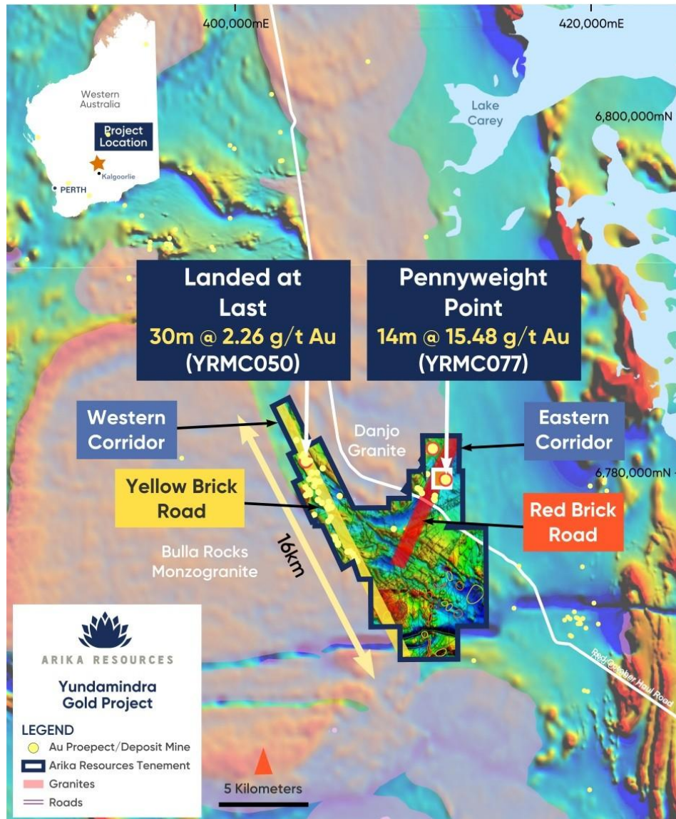
Figure 6: Arika’s Yundamindra Gold Project showing key target areas and prospects over simplified geology, regional and local scale TMI.
