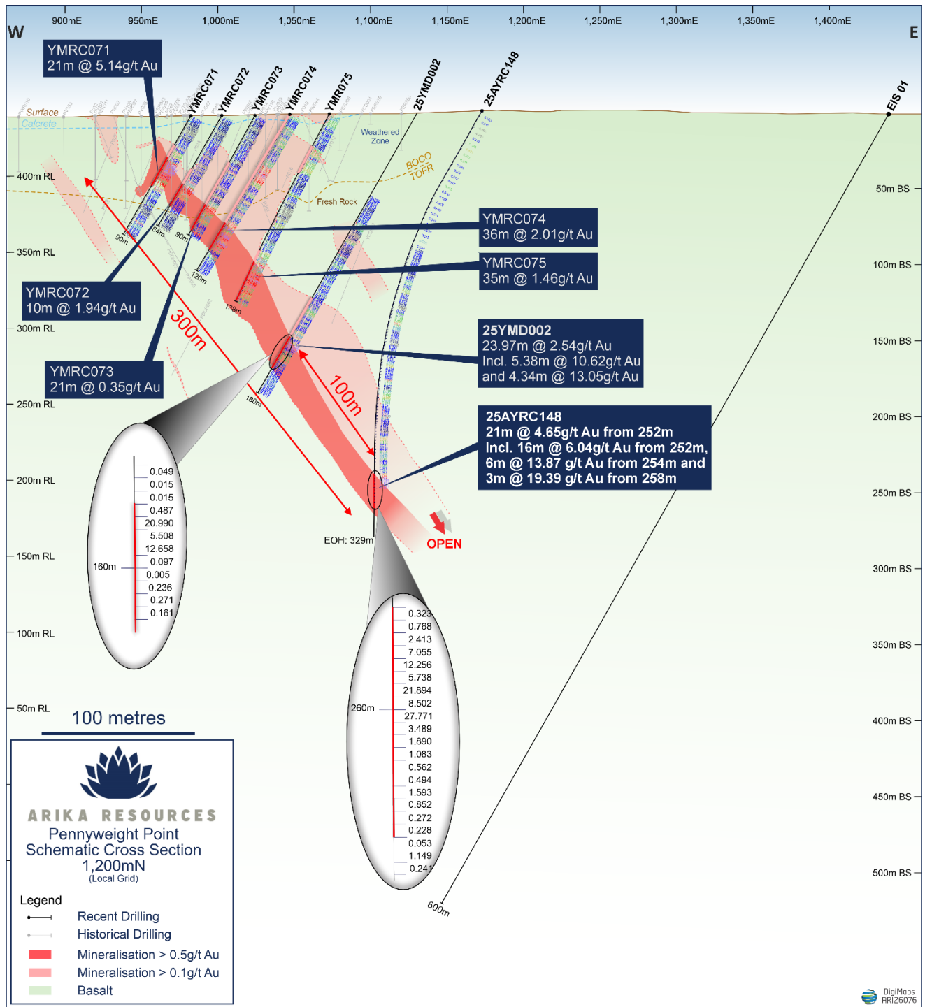
Figure 4: Schematic Cross-Section Line 1,200m N (local grid) showing proposed EIS diamond drillhole P_EIS01 in relation to Arika's most recent drilling and historical holes. Note: Drillhole 25AYRC148 is currently the deepest drillhole completed anywhere on the Yundamindra Gold Project. 3
