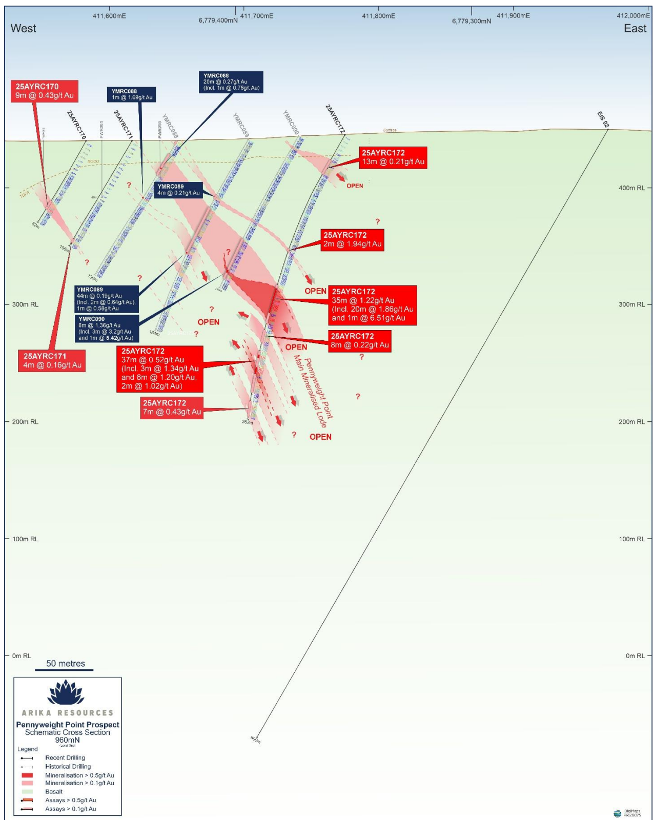
Figure 5: Schematic Cross-Section Line 960m N (local grid) showing proposed EIS diamond drillhole P_EIS02 in relation to Arika's most recent drilling and historical holes. Note: Drillhole 25AYRC172 shows the zone of mineralisation strengthening down-dip of relatively weakly mineralised shallow holes. 4
