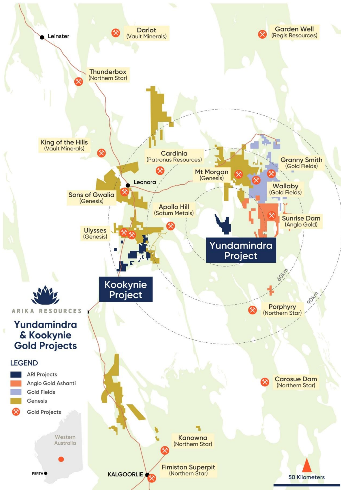
Figure 7: Regional Location Plan: Arika's Kookynie and Yundamindra Gold Projects in relation to major mines, deposits, processing facilities and established infrastructure.
