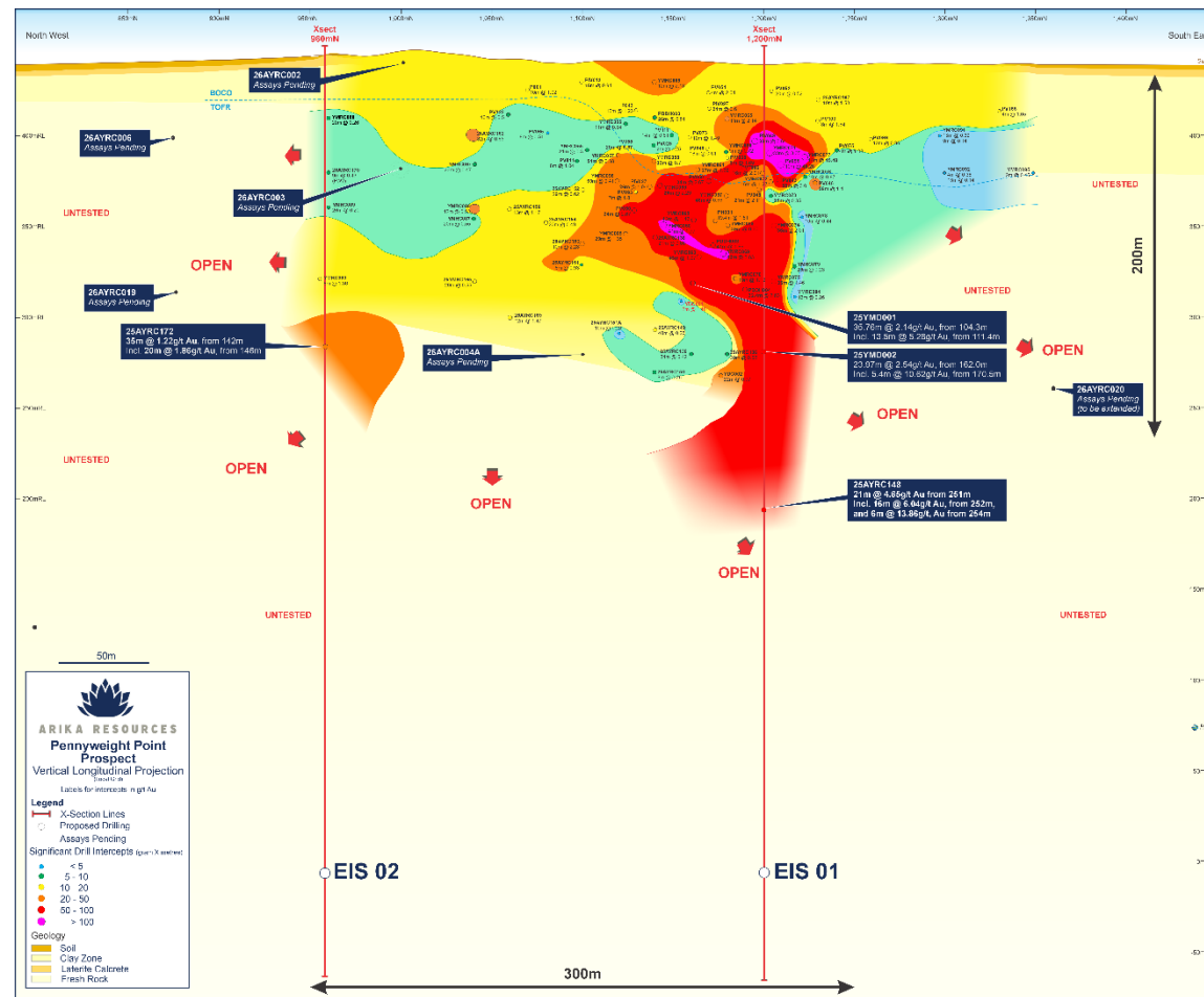
Figure 3: Zoom-in Vertical Longitudinal Projection of the Pennyweight Point prospect showing the location of two proposed EIS diamond drillholes in relation to previous drilling.
