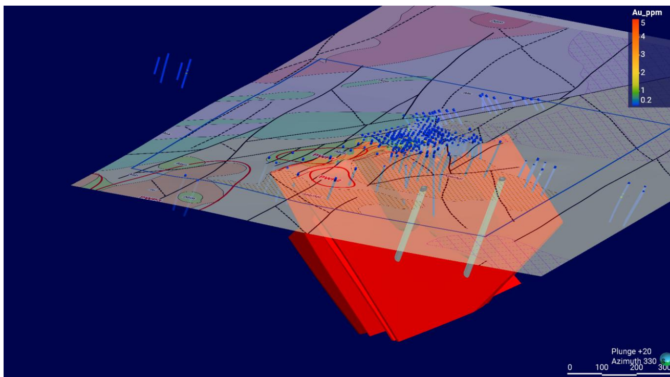
Figure 1: Pennyweight Point 3D model looking north showing the approximate location of two proposed deep EIS diamond drillholes designed to test depth extensions to the near-surface gold-copper mineralisation.
