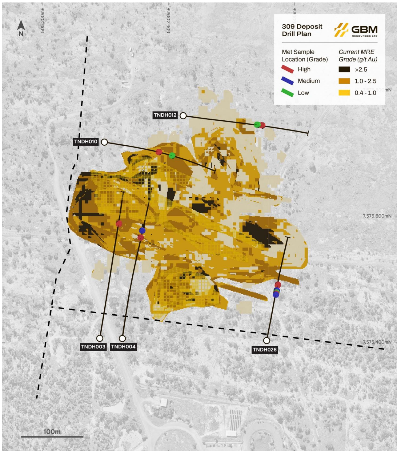
Figure 1 - 309 deposit plan view showing the distribution of metallurgical sample intervals.
