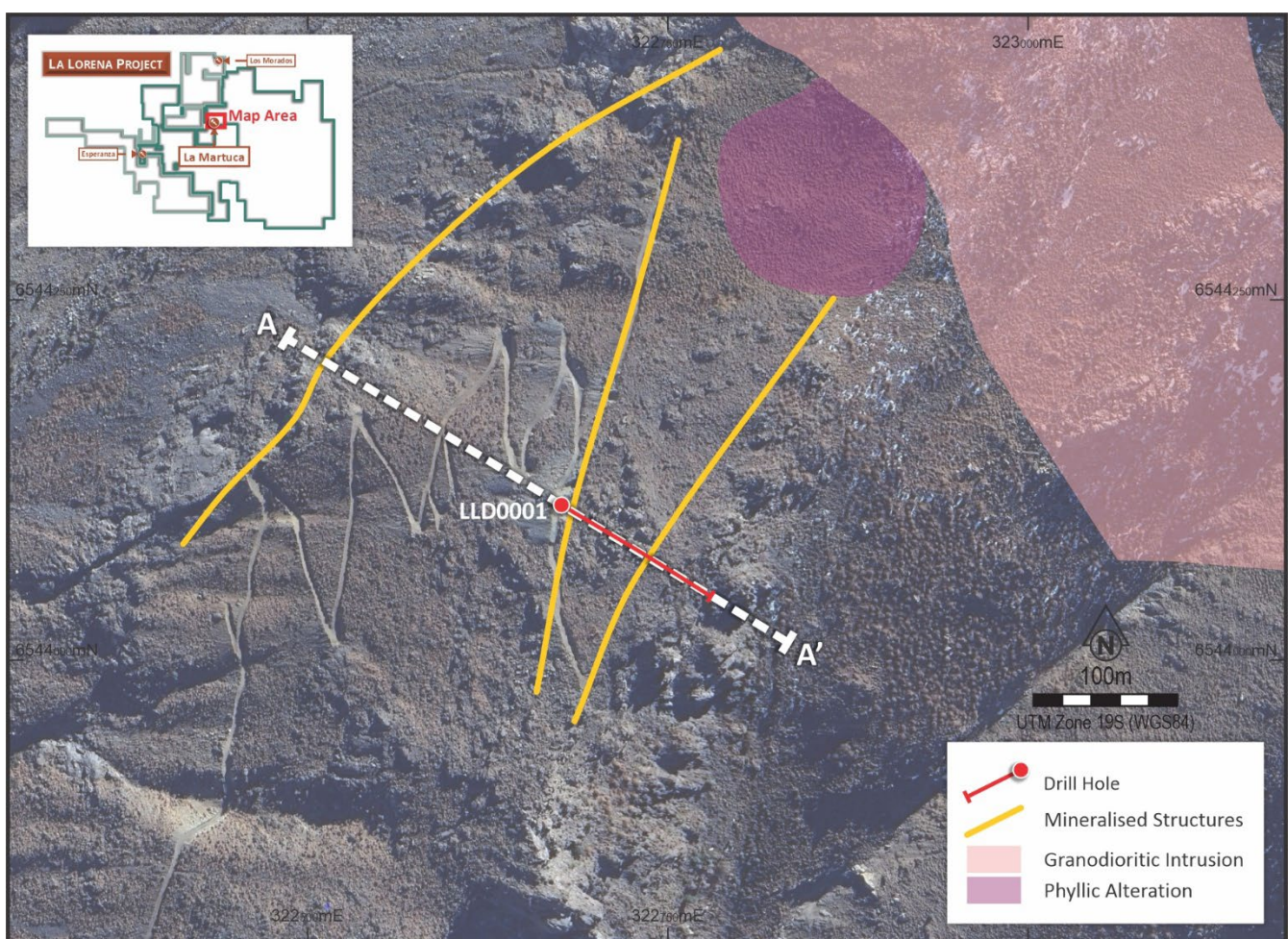
Figure 1. Plan view of the La Martuca prospect showing the location of LLD0001 in relation to the mapped mineralised structures and geological mapping at surface.
