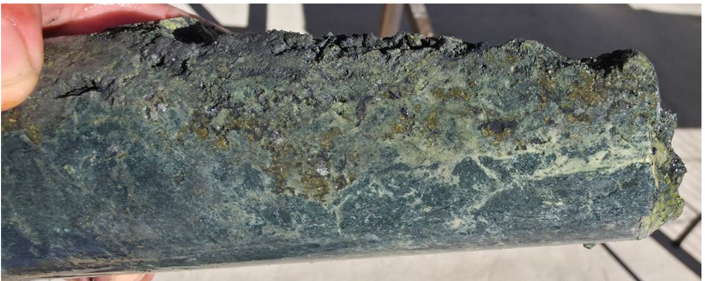
Photo 2. Chalcocite and chalcopyrite in the 20.95–22.6m structure, LLD0001.
