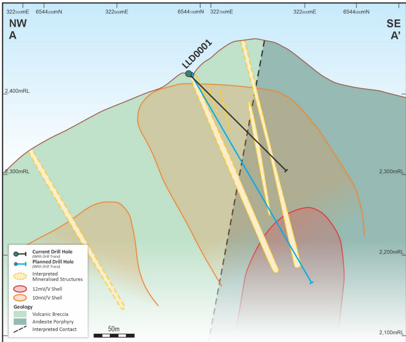
Figure 2. La Martuca cross-section showing LLD0001 to current depth, interpreted extensions of intersected mineralised structures and chargeability target for the second drill hole
