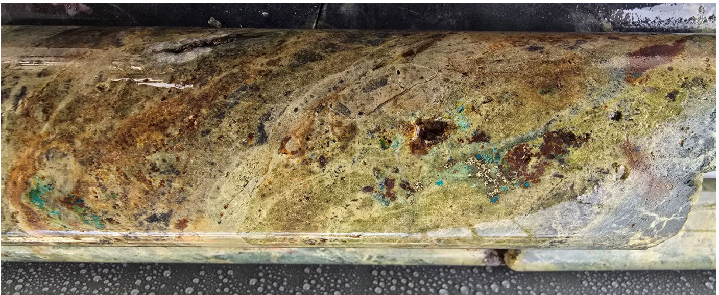
Photo 4. Oxidised quartz-epidote-chlorite structure with chrysocolla and leached pyrite from 63.4–64.35m, LLD0001.
