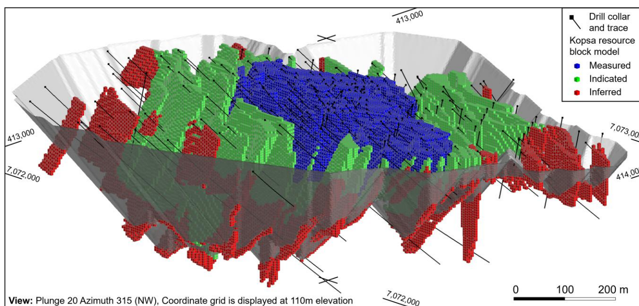
Figure 1. View to the NW of the Kopsa block model shaded by resource classification and the associated optimised pit shell. Coordinates presented in ETRS-TM35FIN system (EPSG:3067).
