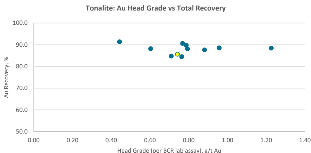
Figure 2: Gold recovery plot showing Tonalite variability tests vs LCT-2. The yellow dot shows the LCT-2 result.
