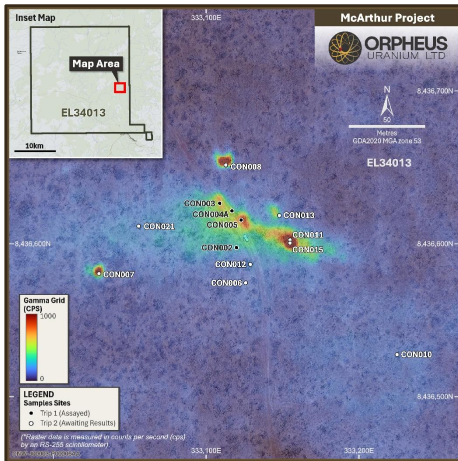
Figure 3: Grid of total count radiometric results associated with data captured during ground based radiometric survey
