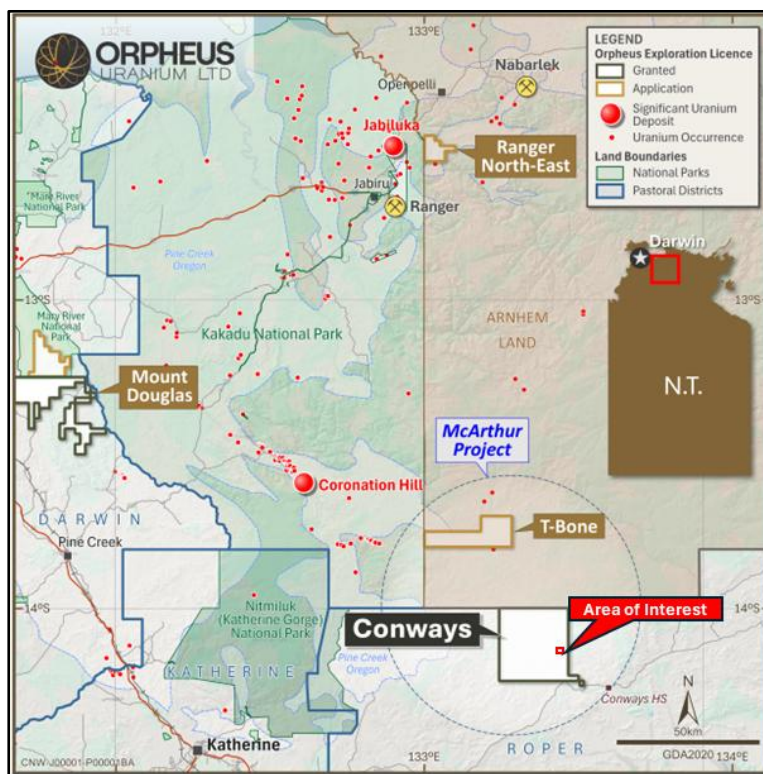
Figure 2: Location of the McArthur Project, Conways tenement and associated area of interest.
