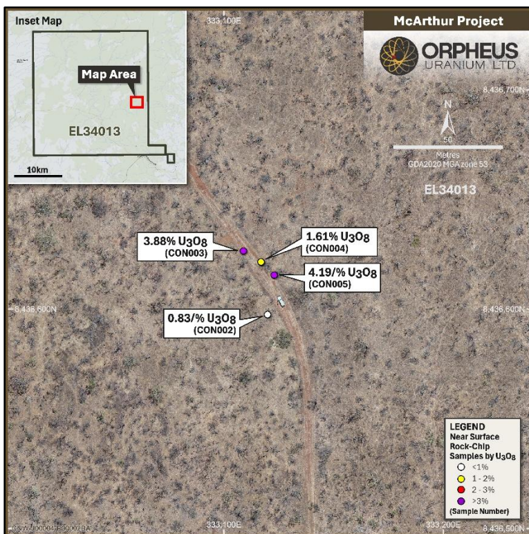
Figure 1: Sample location of near-surface geological samples with U 3 O 8 % analysis and sample ID (reference Table 1 and 2).
