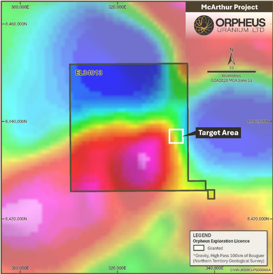
Figure 5: Regional gravity grid over the Conways tenement (sourced: NTGS)
