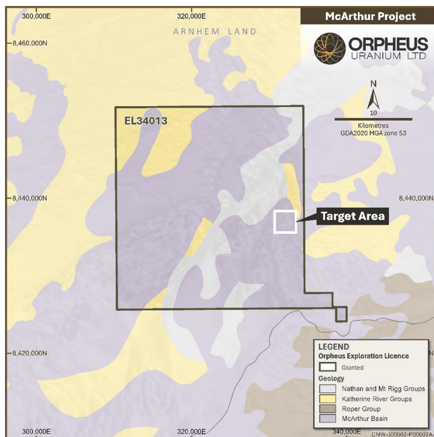
Figure 4: Geological setting of the broader Conways tenement.
