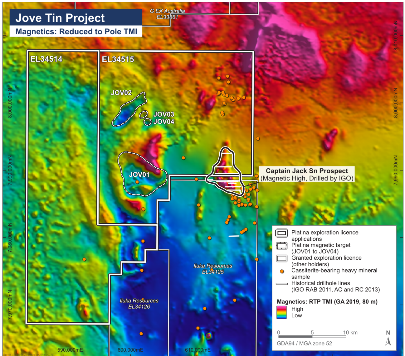
Figure 3 Regional Reduced to Pole total magnetic imagery identifying JOV01–JOV04, historical drilling, regional cassiterite occurrences and Jove tenement boundaries abutting tenements held by Iluka Resources.
