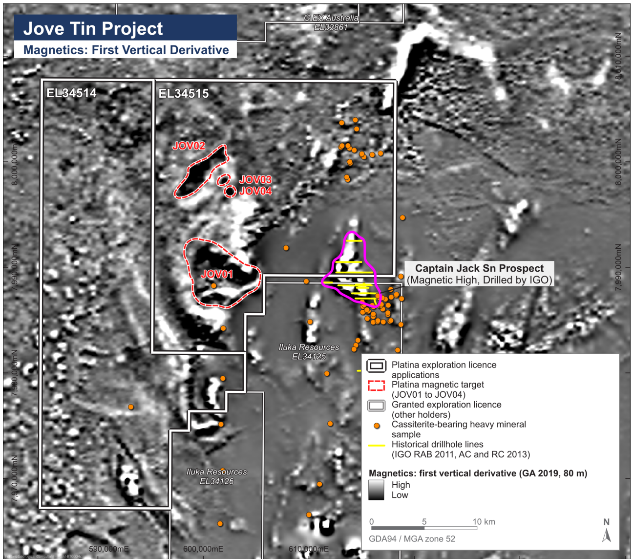
Figure 4. Regional First Vertical Derivative magnetic imagery identifying JOV01–JOV04, historical drilling, regional cassiterite occurrences and Jove tenement boundaries.
