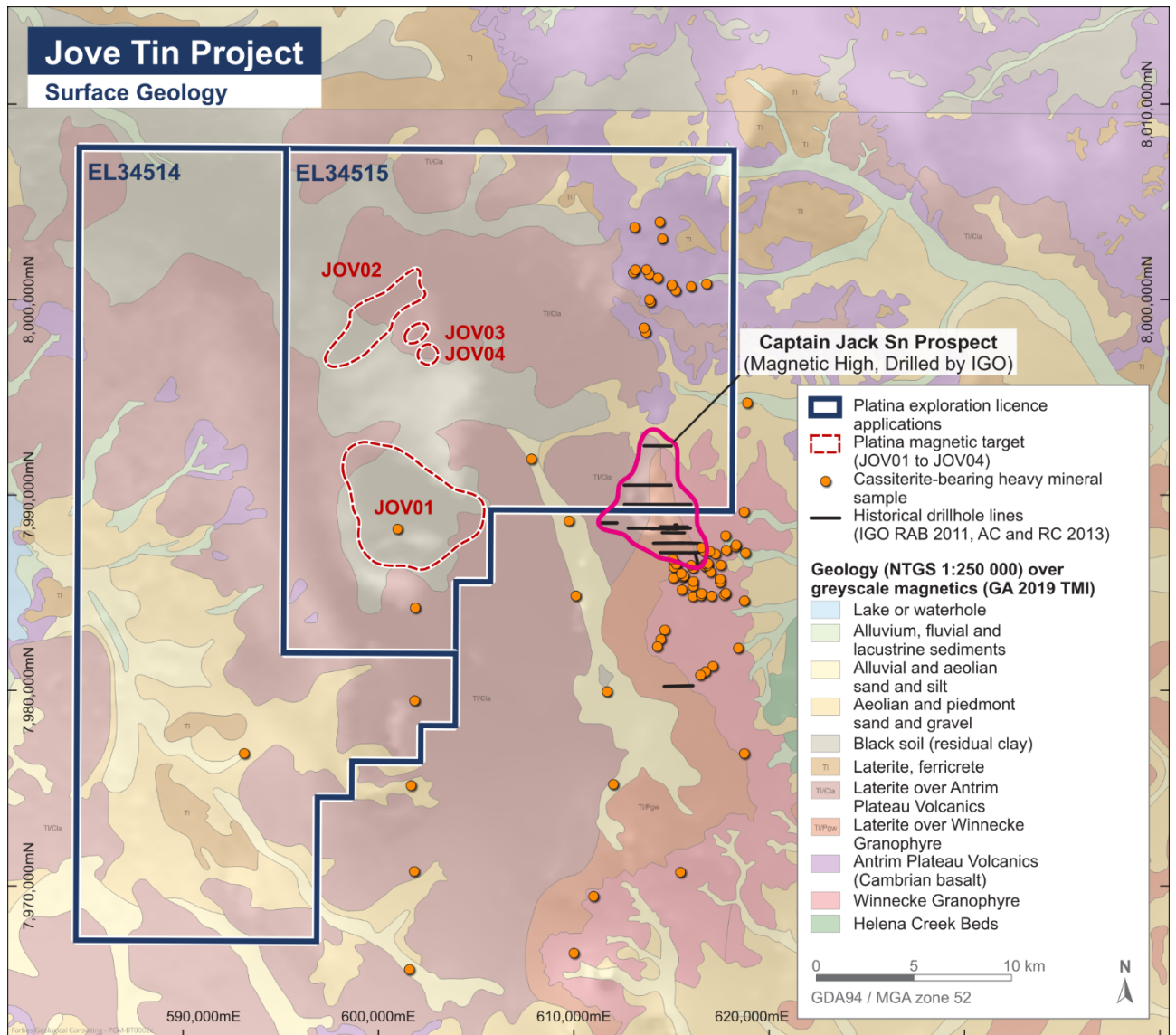
Figure 2: Historical cassiterite occurrences, regional geology, Captain Jack prospect and Jove licence applications.
