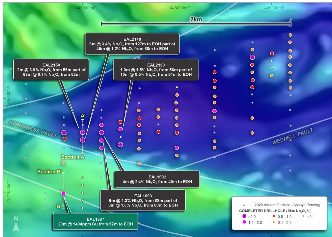
Figure 1 –Joyce Plan (Magnetics TMI 1vd) – High-grade niobium zone continuous over three sections and zone of copper anomalism at Joyce.
