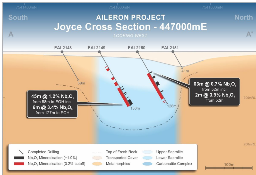
Figure 2 - Joyce 447000E Cross Section A - A'
