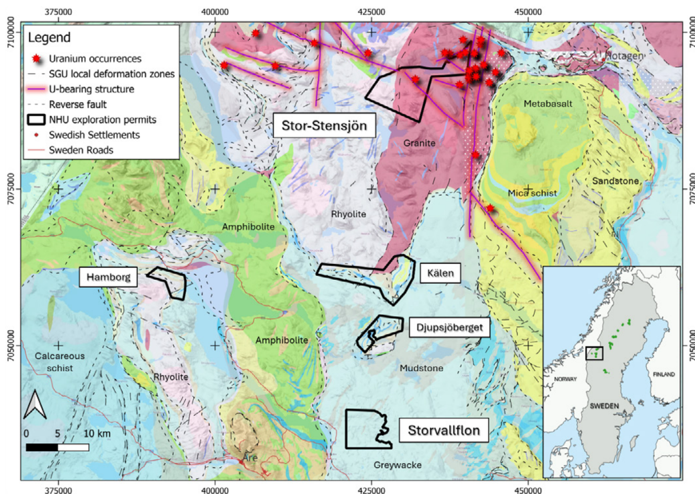
△ Figure 3 Location of the Stor-Stensjön and Storvallflon prospects within Neu Horizon's Hotagen and Krokrom projects respectively, where RadonX™ surveys were planned.
