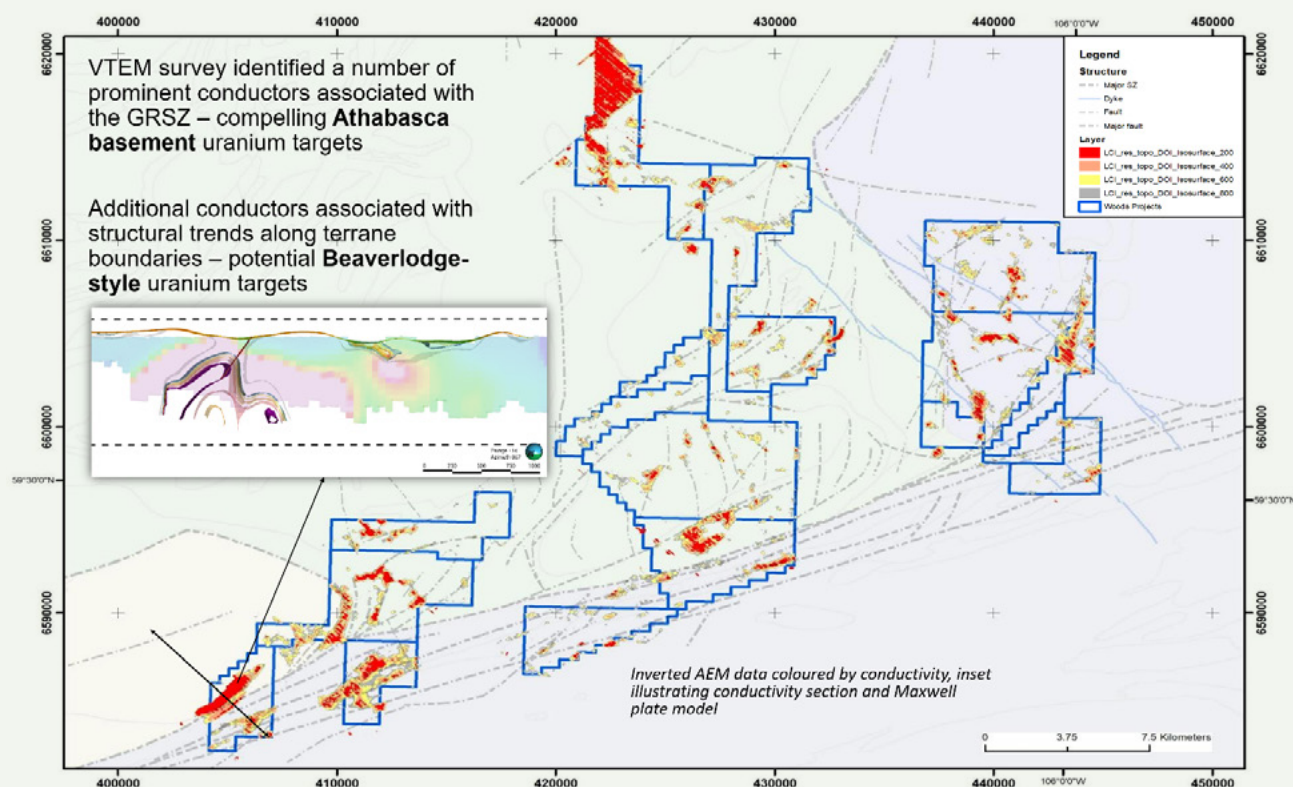
△ Figure 7 Significant VTEM anomalies delineated along the GRSZ from the EM survey flown by Geotech Ltd in September-October 2025
