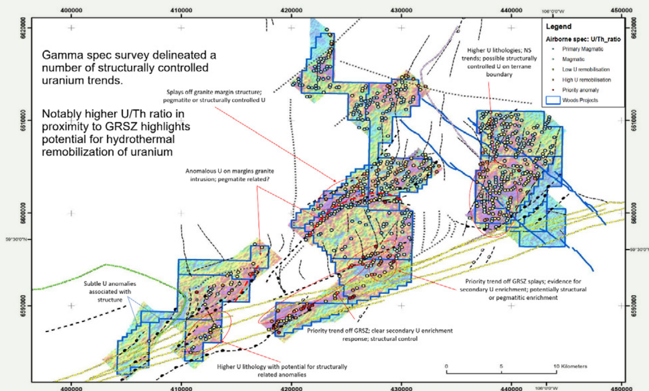
△ Figure 6 Significant radiometric anomalies delineated from the radiometric survey flown by GeoTech Ltd in September 2025
