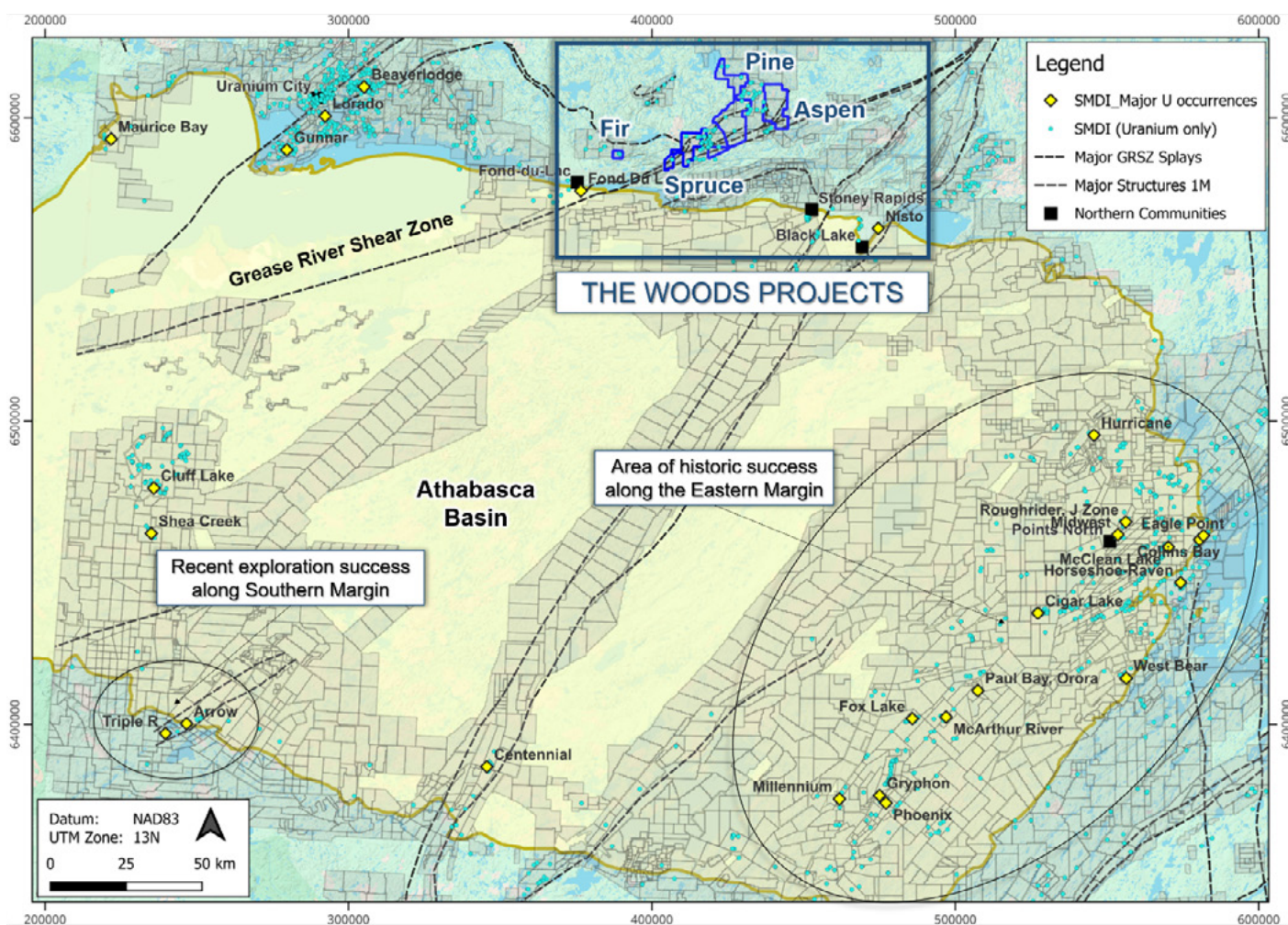
△ Figure 5 Location of Neu Horizon's Woods Projects along the northern margin of the Athabasca Basin, Saskatchewan
