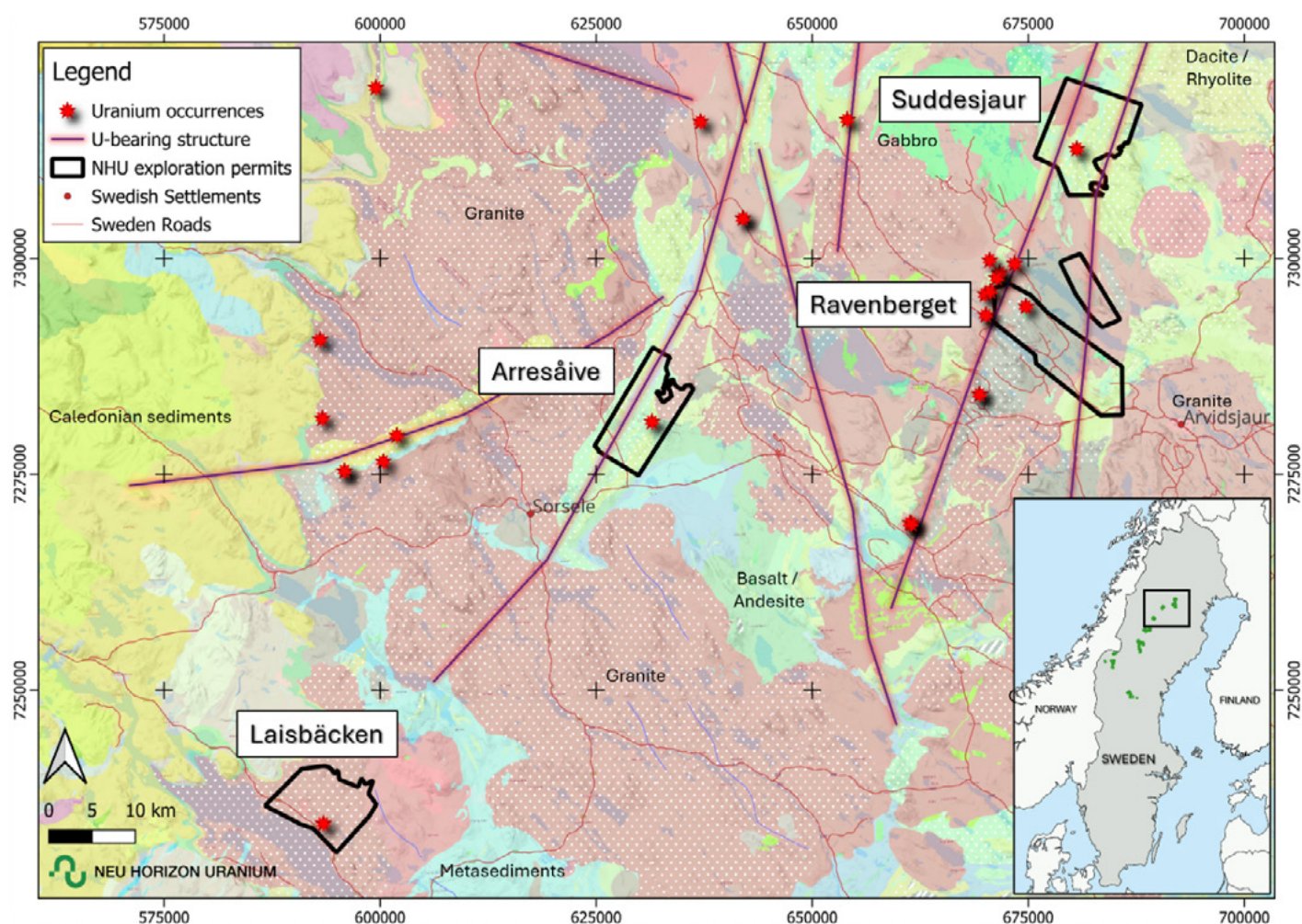
△ Figure 1 Location of Neu Horizon's Arvidsjaur prospects
