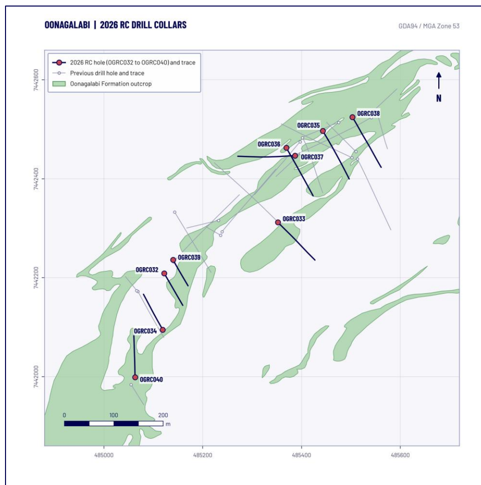
Figure 1. The 2026 RC holes OGRC032-OGRC040 shown with previous drilling over the mapped outcrop of the Oonagalabi Formation. Coordinates are GDA94 / MGA Zone 53. 2
