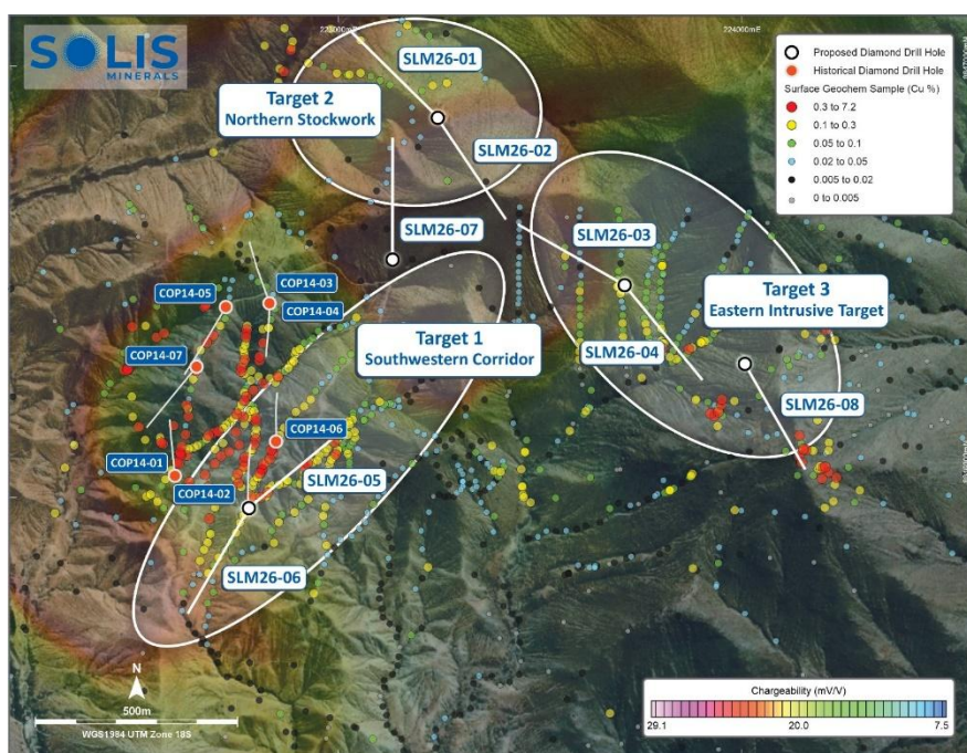
Figure 1: Cucho exploration area – target zones indicated with historical drillhole collars and traces, planned drill holes and traces, copper surface geochemistry and IP chargeability.
