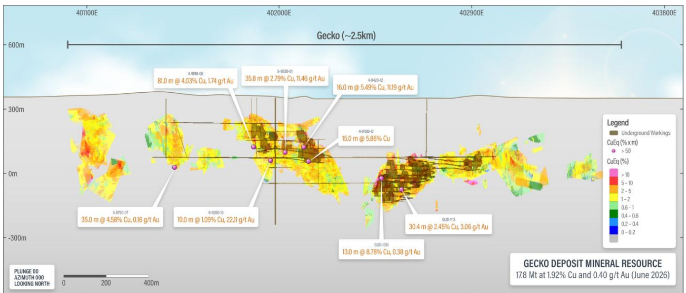
Figure 3: Long section of Gecko deposit.
