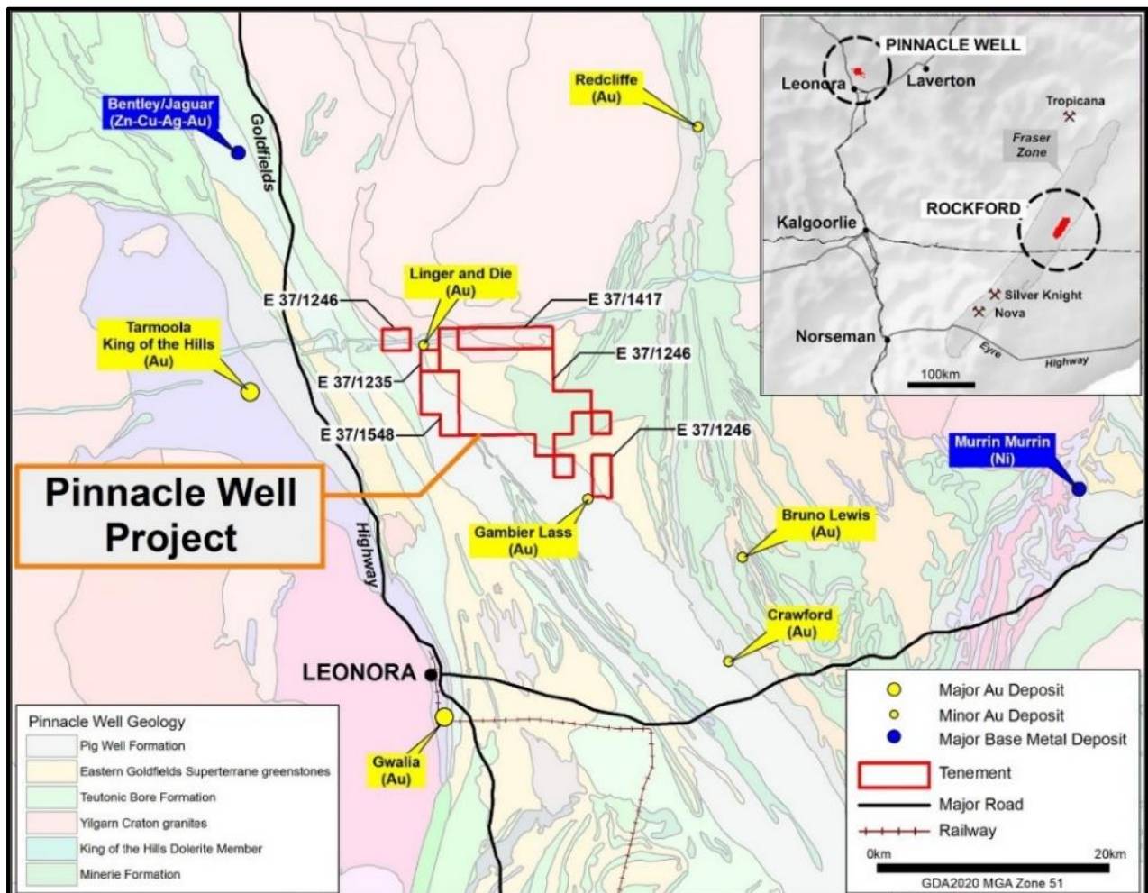
Figure 2: Pinnacle Well Project with Major Mines/Deposits on Regional Geology (GSWA 1:500K)
