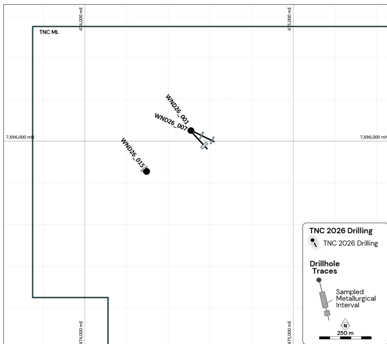
Figure 10: Collar locations for Wallace North DD metallurgical drilling completed by TNC in 2026
