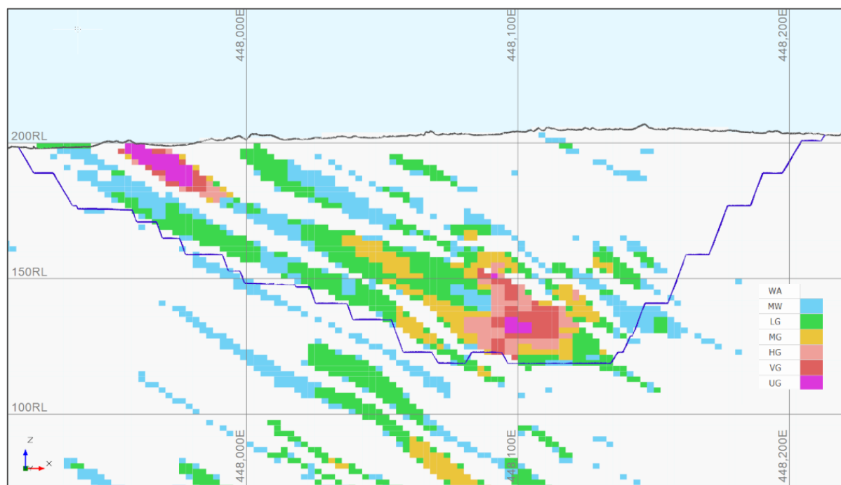
Figure 8: Mongoose-Taipan Pit Design, Cross section through 7,708,340 mN, looking North
