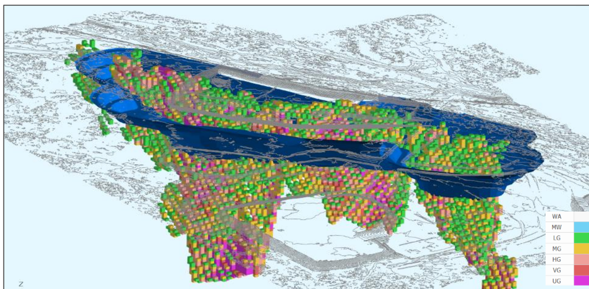
Figure 7: Wallace North Pit Design and Resource Model, Oblique view looking south-east
