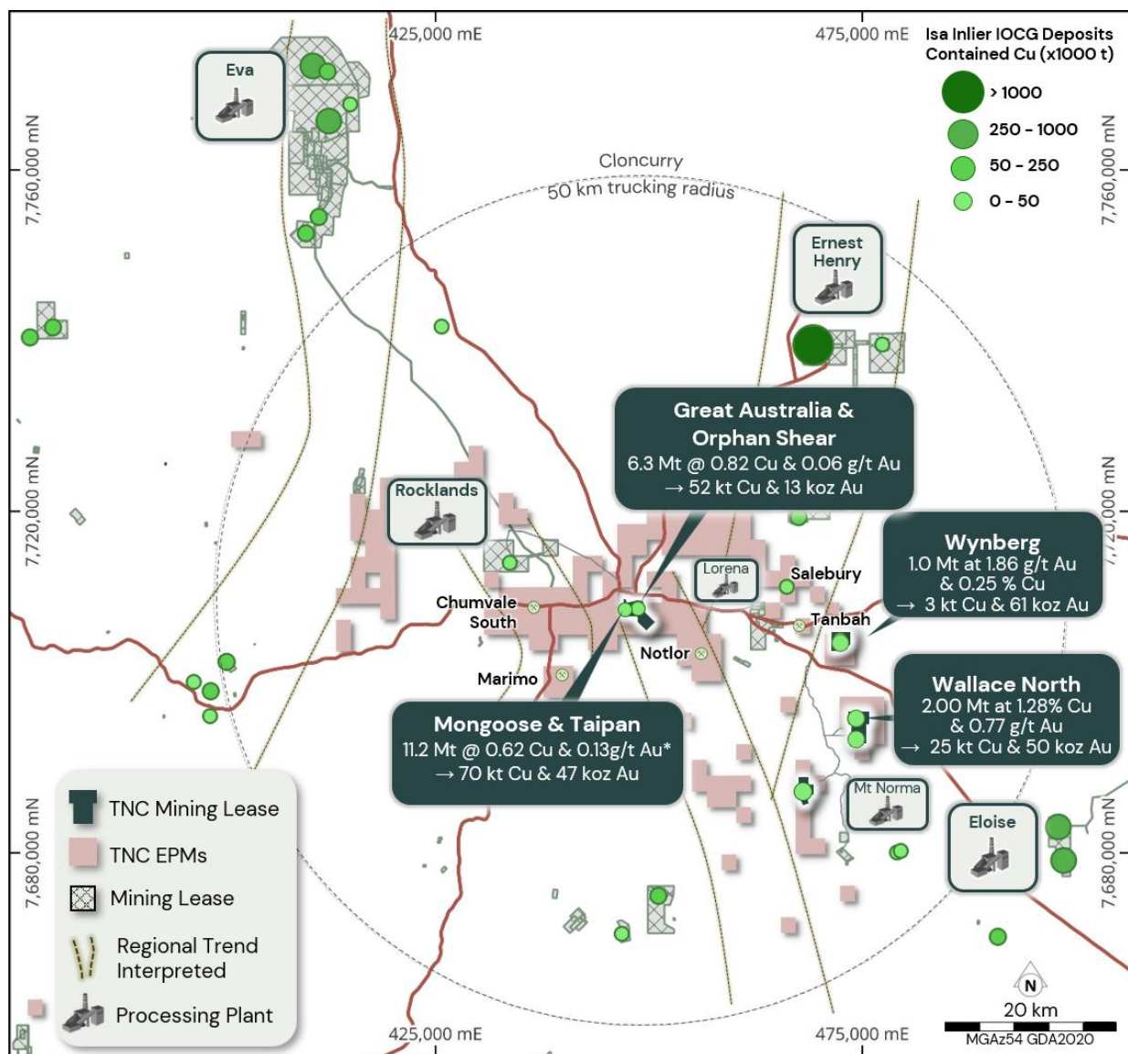
Figure 3: TNC's Cloncurry Copper Project within context of other regional district copper resources
