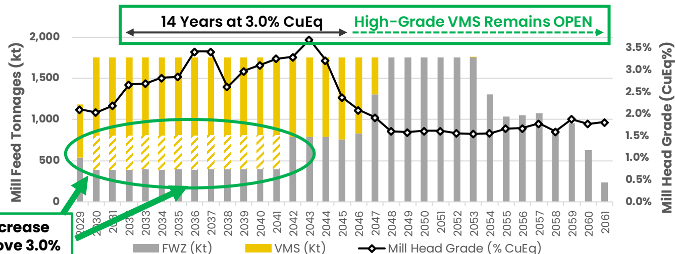
Mill Feed by Mineralization Type - 1.8 Mtpa Case
