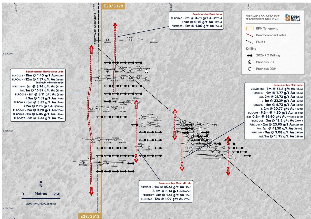
Fig. 2 - Beachcomber Prospect plan view showing the Main, North-West, Central and Fault Lodes and the 2026 resource definition drilling
