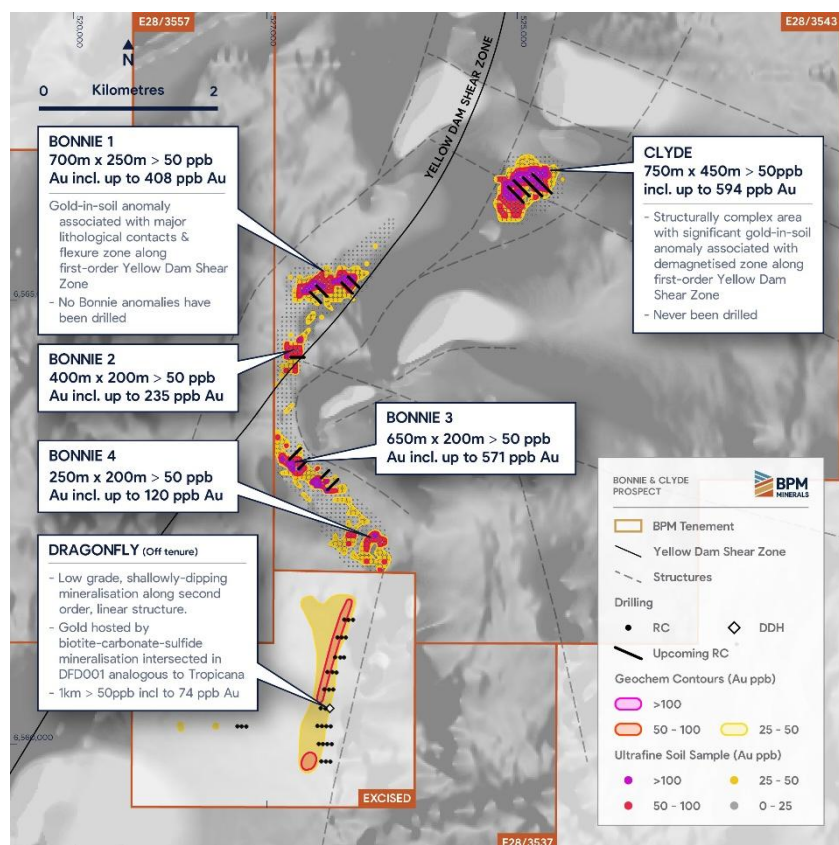
Fig. 3 - Bonnie & Clyde ultrafine fraction gold-in-soil anomalies over airborne magnetics, showing the Clyde, Bonnie 1, Bonnie 2 and Bonnie 3 targets and planned RC drill holes
