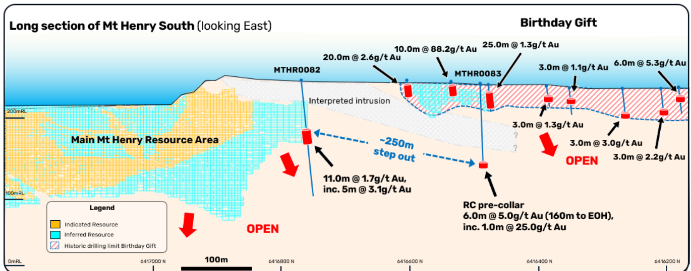
Figure 4: Significant gold intersections beyond the southern Mt Henry Resource boundary, including high-grade mineralisation beneath the interpreted intrusion towards Birthday Gift.
