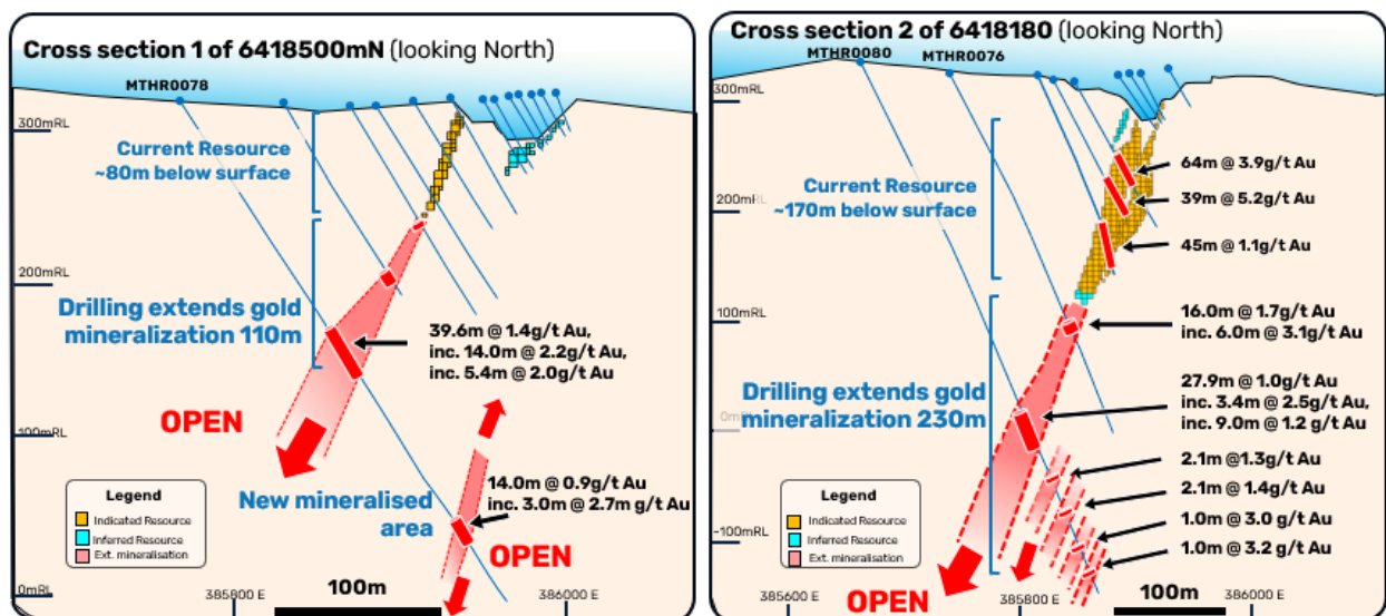
Figure 1: Broad gold intersections extend mineralisation up to 230m beyond the current Resource and identify new mineralised zones within the northern portion of the Mt Henry deposit.
