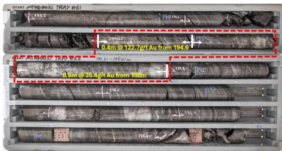
Figure 2: Exceptional high-grade gold intersections of 0.4m @ 122.7g/t gold and 0.9m @ 35.4g/t gold, associated with quartz-sulphide veining in sulphidised BIF (MTHD0021).
