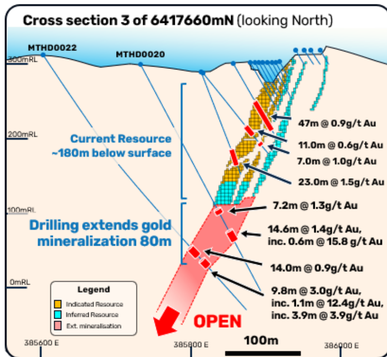
Figure 3: Broad, high-grade gold intersections extend mineralisation 80m beyond the current Resource at central Mt Henry, highlighting further growth potential at depth.
