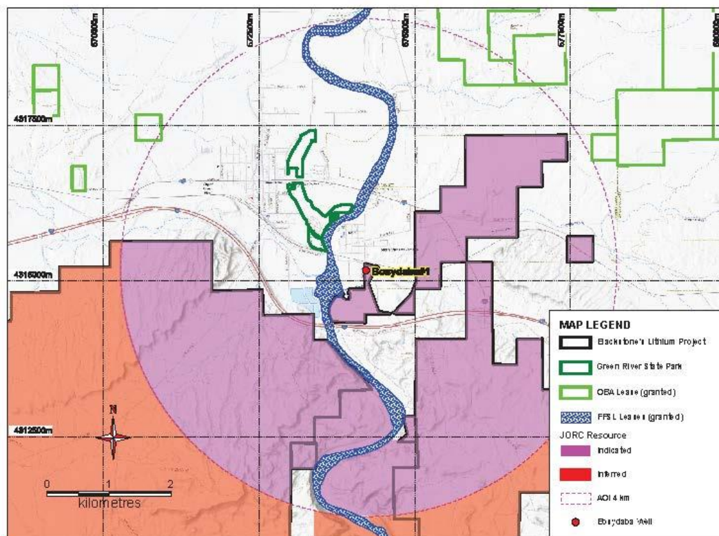
Figure 1: Plan showing the State Park blocks applied for at its Green River Lithium Project.
