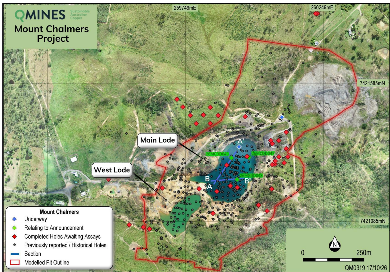
Figure 2 - Collar locations, Mt Chalmers.
