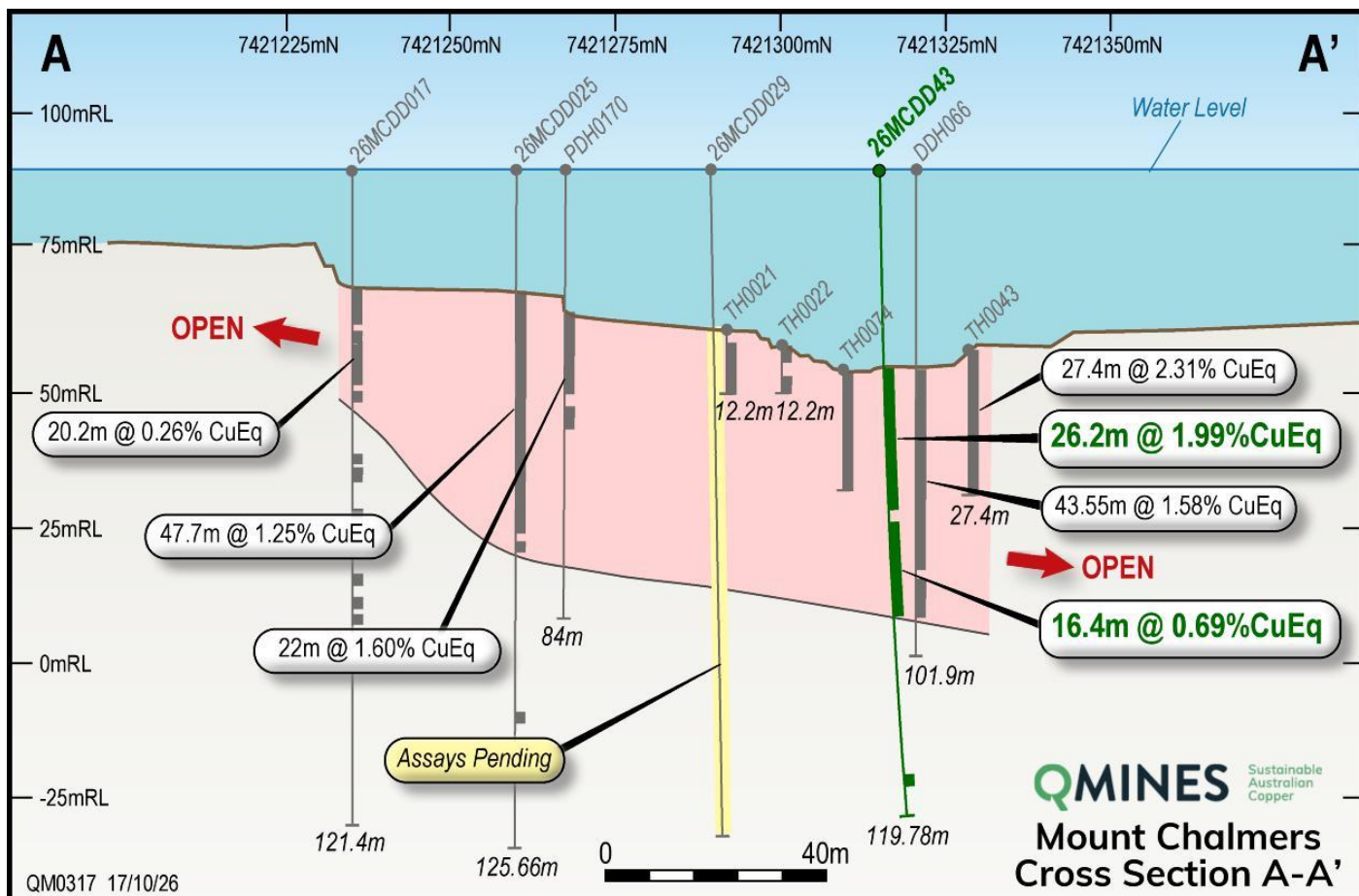
Figure 3 – A-A'; cross-section on a 12.5m window thickness illustrating the mineralised envelope.
