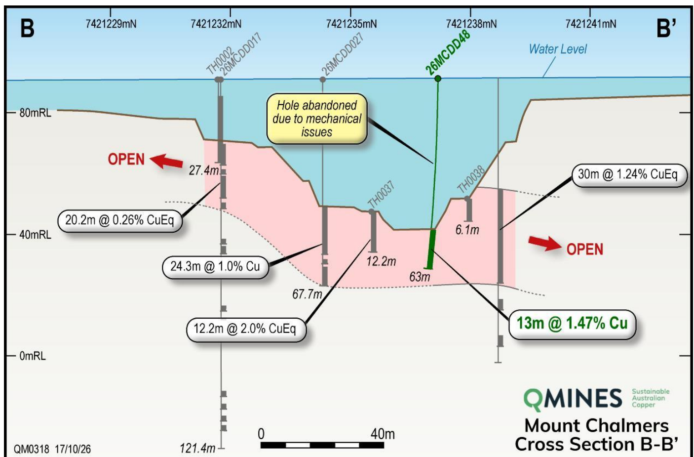
Figure 4 – B-B'; cross-section on a 12.5m window thickness illustrating the mineralised envelope.
