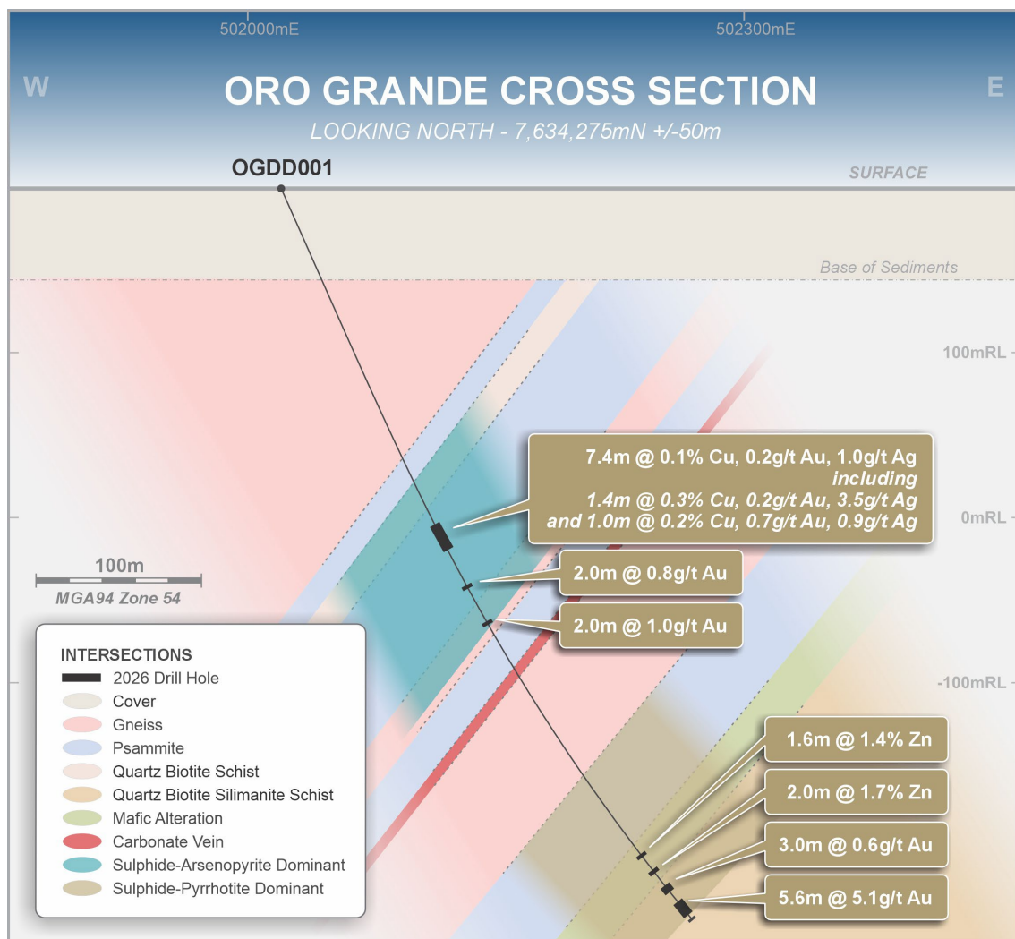
Figure 3. Oro Grande cross section showing drill hole and interpreted geology.
