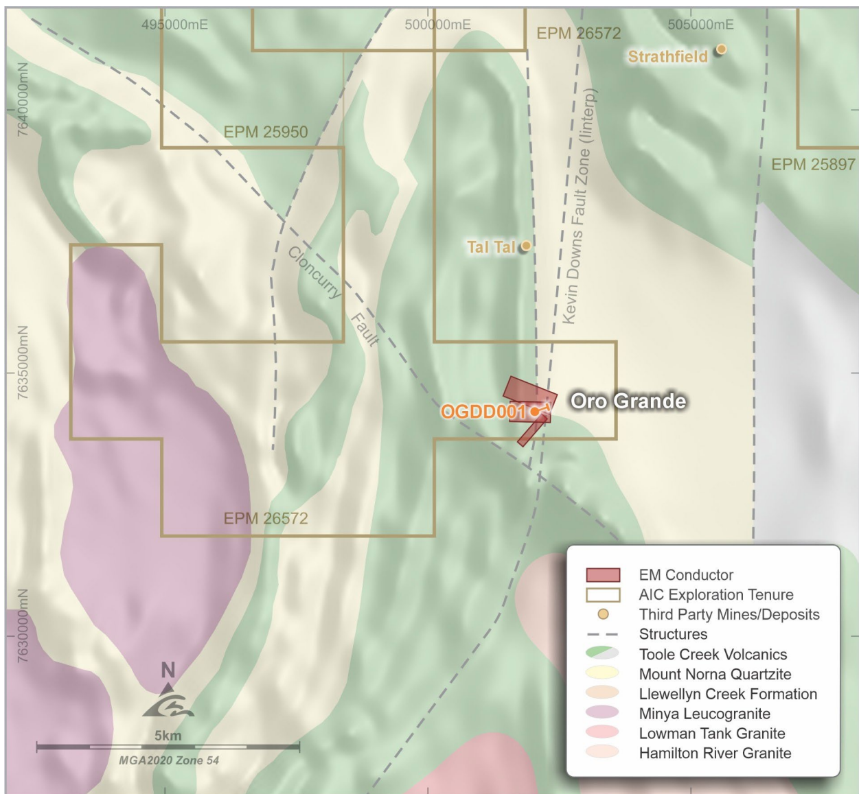
Figure 2. Location plan showing the Oro Grande drill hole in relation to the GEM conductors.
