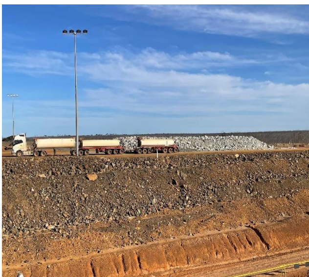
Figure 7: Stockpiles established on the Cosmic Boy ROM pad ahead of commencement of processing.
