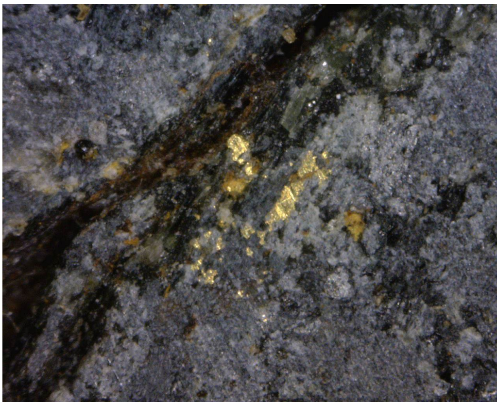
Figure 1: Visible gold grains in an outcrop sample from Jukulainen that returned an assay result of 43.7g/t Au. Field of view in this photo is 3 x 2.5mm. The host rock is a mafic/intermediate volcanic and the visual estimate of the amount of gold in the sample is less than 1%. For full sample details please refer to Appendix 1.
