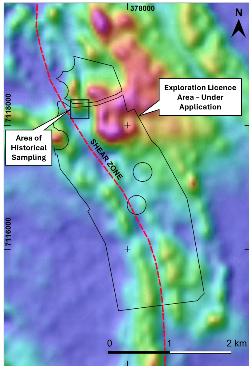
Figure 3: Jukulainen tenement map over regional magnetics. Magnetic map (Red = Magnetic High) is from the Geological Survey of Finland ("GTK") database. Coordinates provided in ETRS-TM35FIN system (EPSG:3067).
