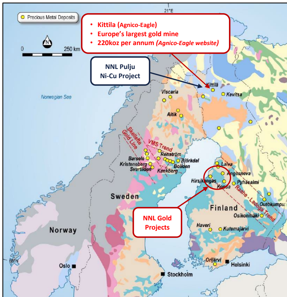
Figure 5: Location of NNL's gold projects shown over a geological map of Finland.
