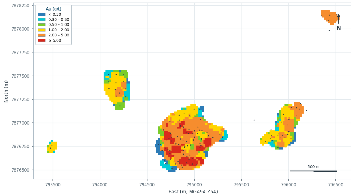
Figure 3-8: Block model plan view - maximum Au grade projection, depleted model, with drill collars.
