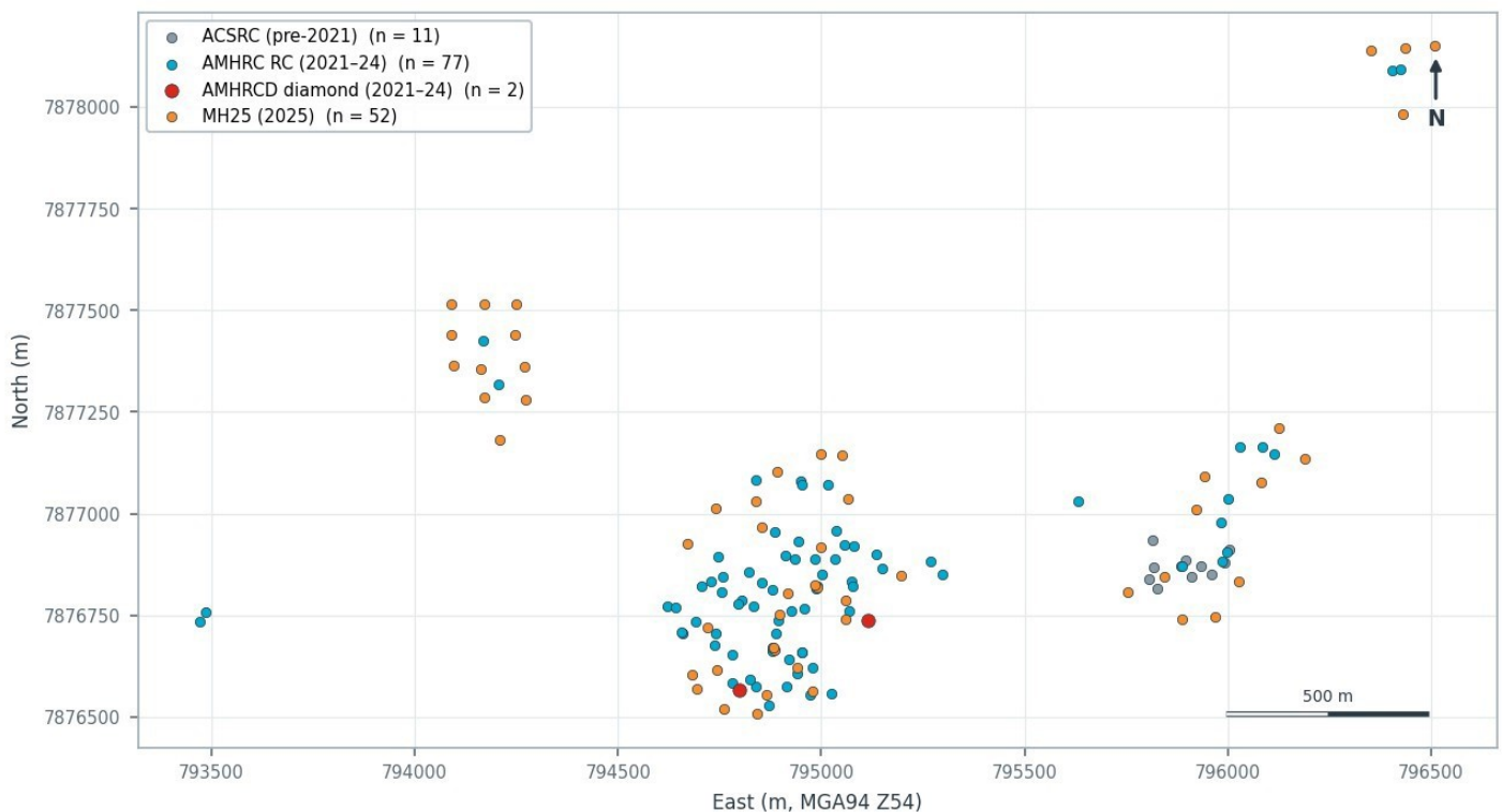
Figure 5. Mt Hogan Project All Drilling
