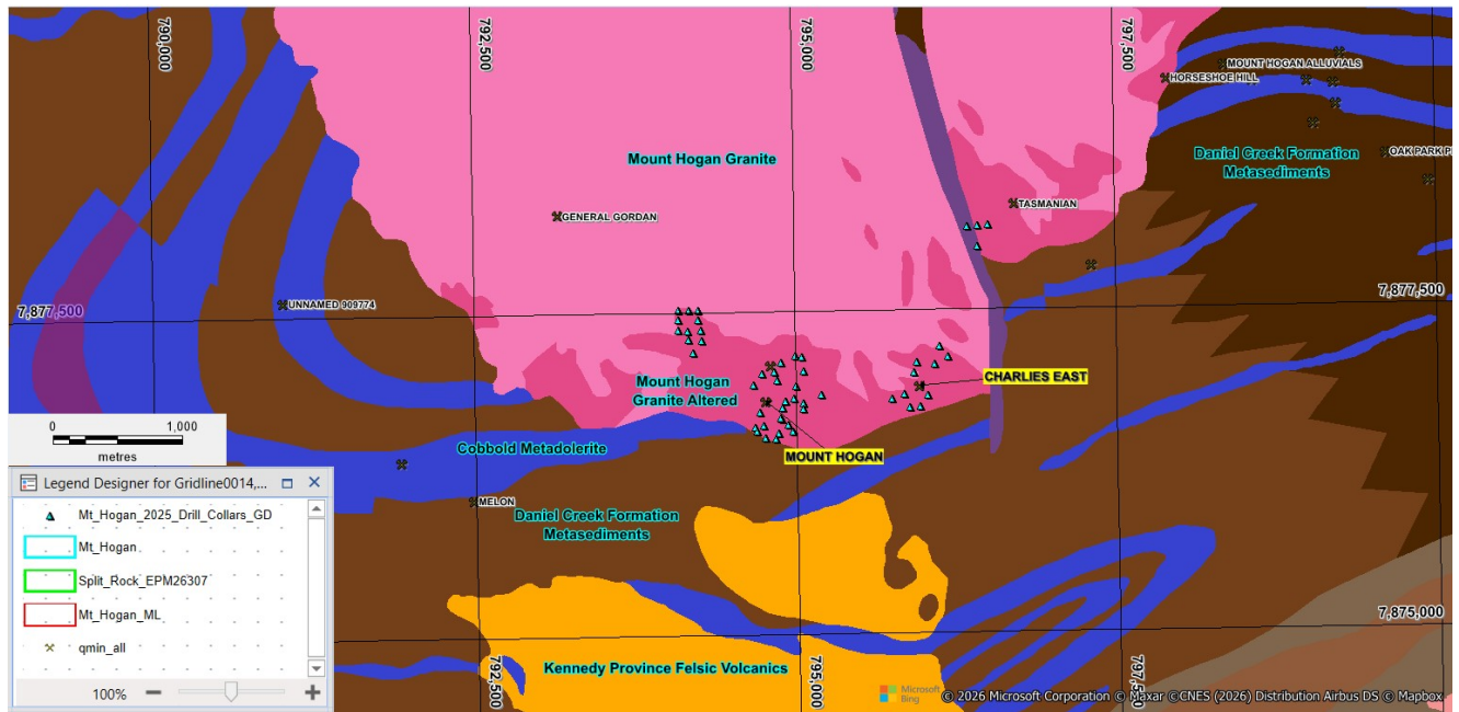
Figure 4. Mt Hogan Project Geology and 2025 RC Drilling
