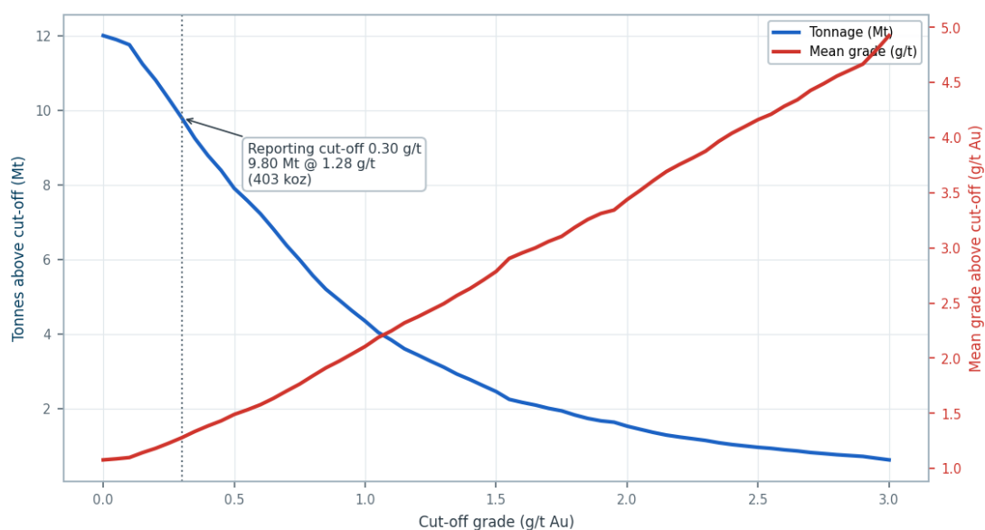
Figure 3-11: Grade-tonnage curve for the depleted model, with the 0.30 g/t reporting cut-off highlighted.
