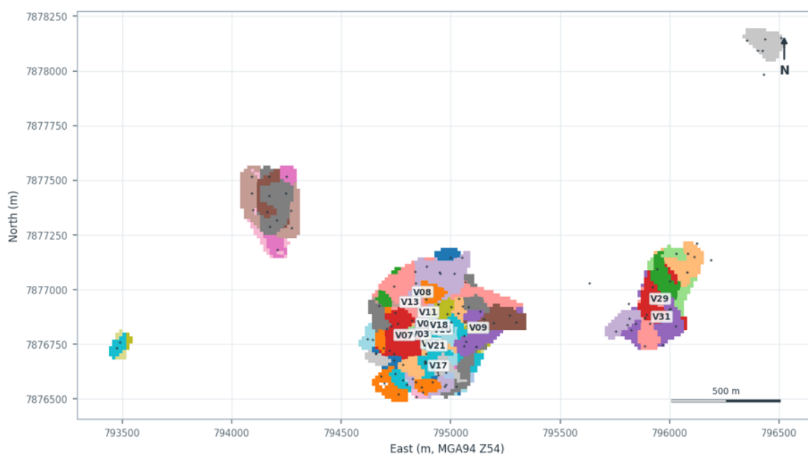
Figure 3-7: Vein domain wireframes: plan projection of the 41 estimated domains, coloured by domain.
