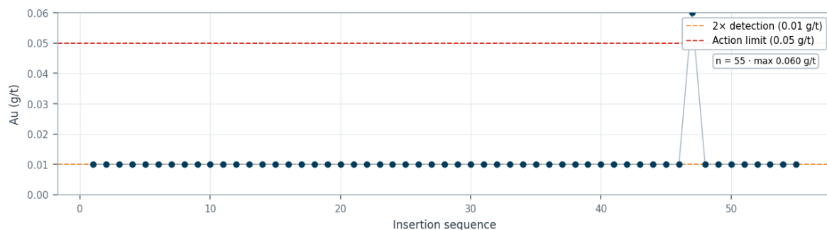
Figure 3-4: QAQC control charts, blank performance.
