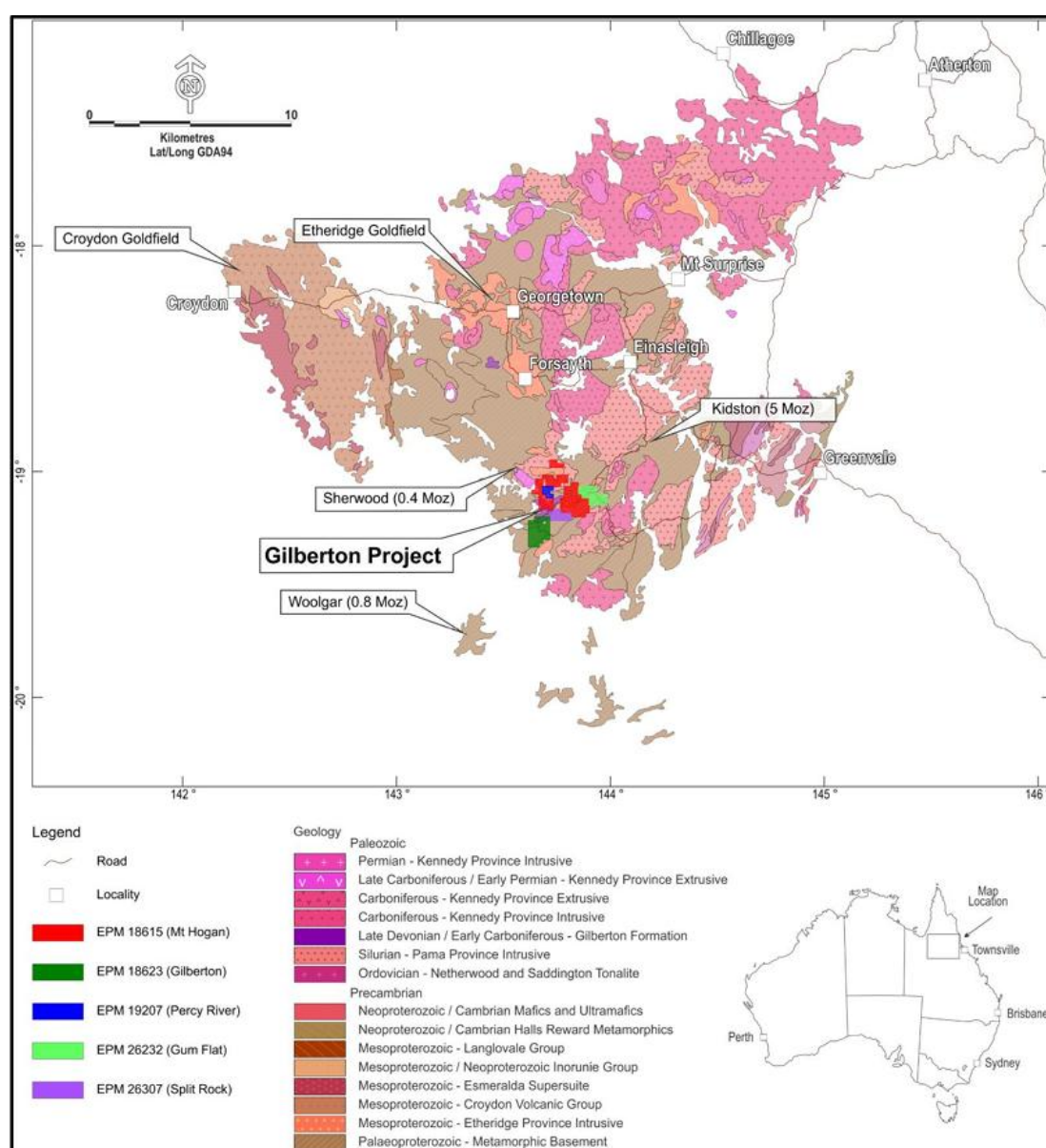
Figure 3-1: Palaeozoic and Precambrian units of the Georgetown Inlier, and location of the Gilberton Gold Project (EPM18615 for Mt Hogan) (Source: Exploration Permit for Minerals 18615. Annual Report 2018).
