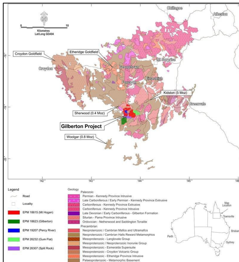
Figure 3. Gilberton Gold Project Regional Geology
