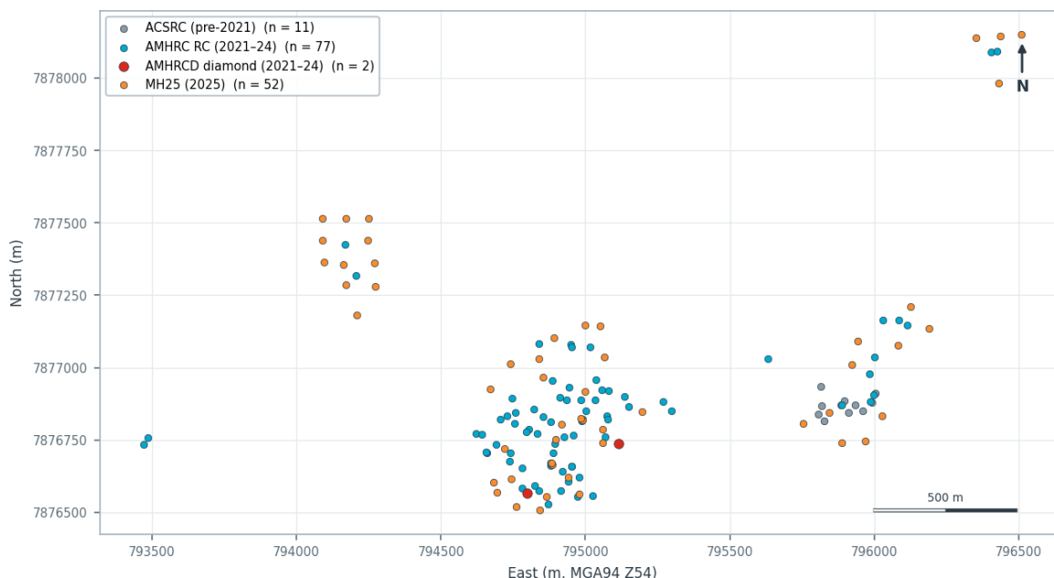
Figure 3-2: Drill collar plan by campaign (142 holes, MGA94 Zone 54).
