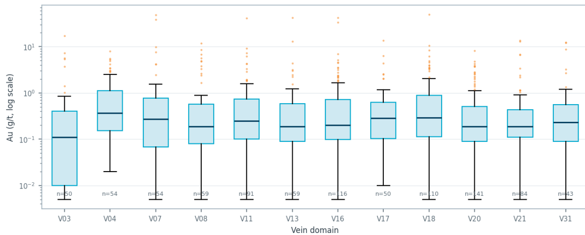
Figure 3-6: Grade distribution by vein domain, twelve largest domains by contained sample metal.
