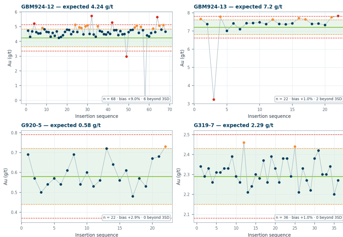
Figure 3-3: QAQC control charts, certified reference material performance, ALS Au-AA25.
