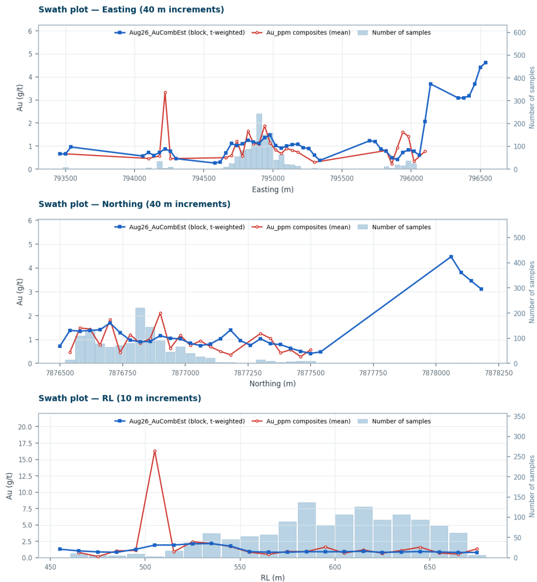
Figure 3-10: Swath plot validation of Aug26_AuCombEst versus in-domain composites, 40 m easting and northing increments, 10 m elevation increments.
