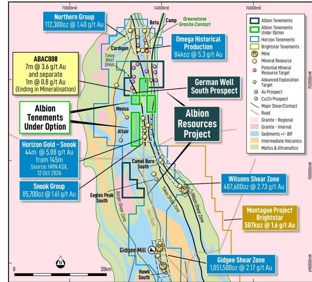
Gum Creek Greenstone Belt
