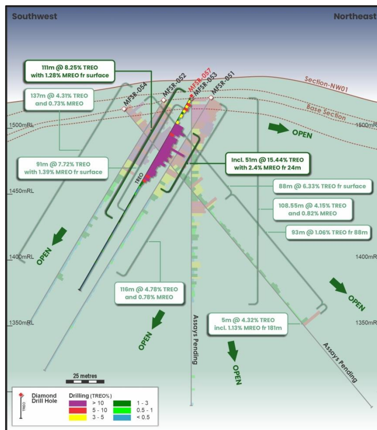
Figure 1. Cross-section looking northwest showing the section with MFSR-057 further up the hill, together with drillholes along the Base Section 5m below and 25m further southeast. The whole-rock TREO percentage is colour-coded on the drill traces. Not all results are available for the lower parts of MFSR-053 and MFSR-054. Results for the Base Section drillholes MFSR-051, MFSR-052, MFSR-053, and MFSR-054 have been disclosed in ASX announcements dated 31 July, 24, 27 August, and 4, 7 September 2026.
