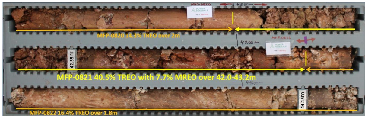
Figure 3. Drill core from MFSR-057 with the extremely high-grade TREO sample MFP-0821, and parts of samples MFP-0820 and MFP-0822 (see Table 3) marked. The material is very fine-grained, soft cream to reddish-brown, clayey phonolite saprolite. Photograph taken dry before cutting the core. Both TREO and MREO are percentage of whole rock analyses. Core recovery was measured at 93.5% between the 41.0m and 42.55m (1.55m interval) core blocks and 100% (no core loss) between the 42.55 and 44.15m (1.6m interval) core blocks. The HQ core shown starts at the top-left, and the downhole direction is to the right; tray rows are one metre long.
