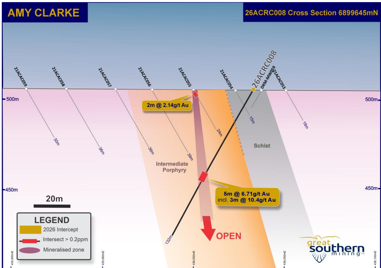
Figure 2. Interpreted cross-section at 6899645mN showing results from recent drill hole 26ACRC008 and previous drilling. Drill hole locations shown on Figure 1 and Figure 4.
