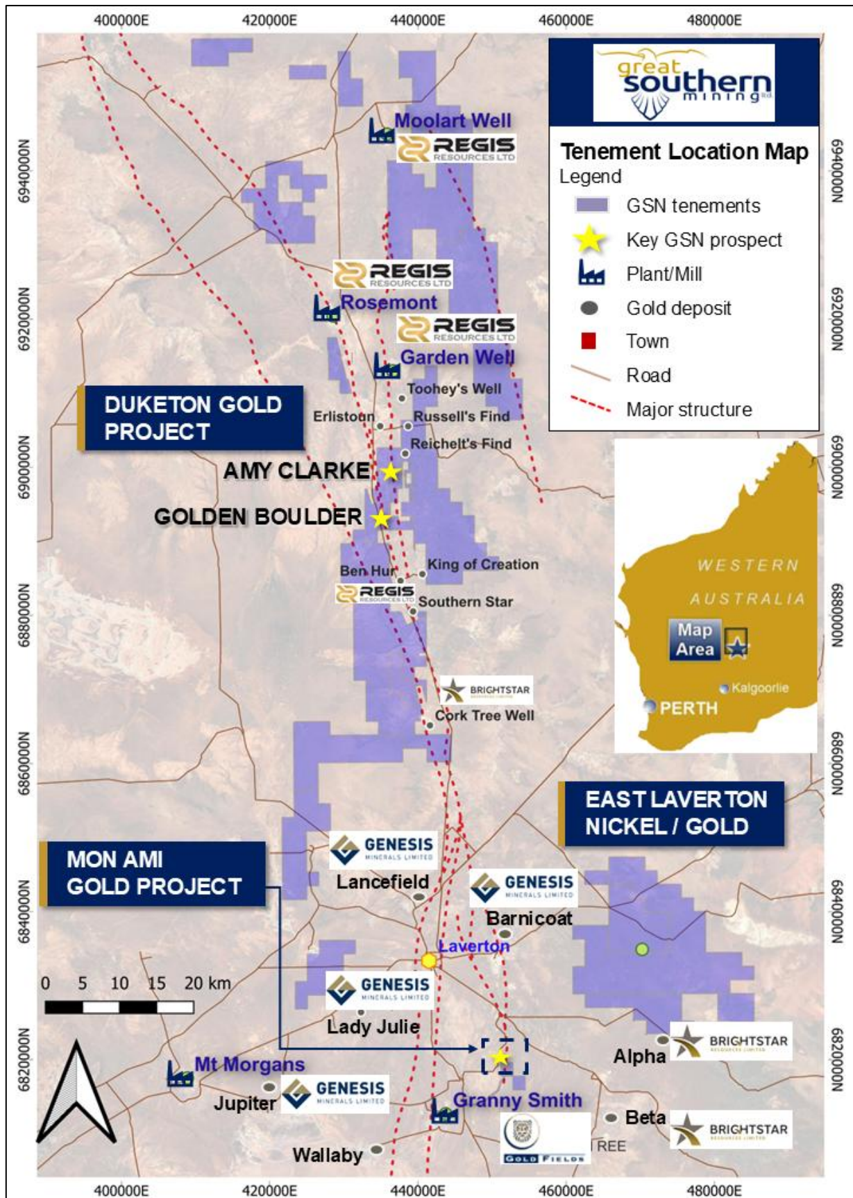
Figure 5. Map of Great Southern Mining's tenure in the Laverton District of Western Australia, incorporating the Duketon Gold, Mon Ami and East Laverton projects, and showing regional mines and processing facilities.
