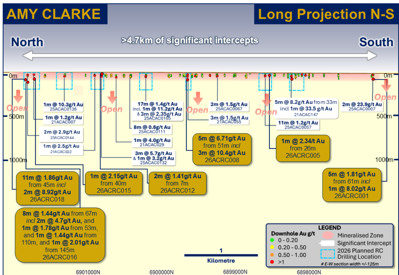
Figure 1. Long projection of the Amy Clarke prospect showing recent significant drill intercepts (in gold) and previous intercepts (in white).
