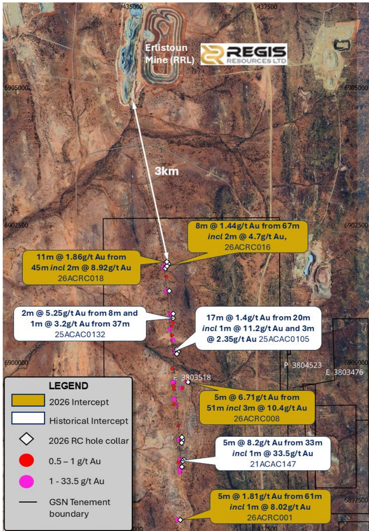
Figure 4. Map showing location of Amy Clarke prospect with significant drill intersections along a north/northwest structural trend along strike from Regis Resources Erlistoun mine (320koz @ 1.9 g/t Au).
