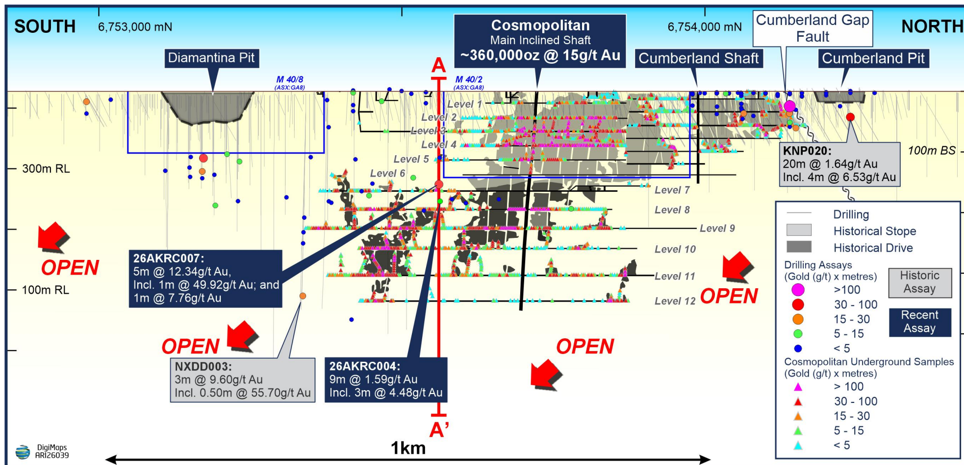
Figure 2: Vertical Longitudinal Projection of the Historical Cosmopolitan Gold Mine 'D-C-C Trend' showing recent drilling in relation to the old workings and previously reported historical underground channel sampling and drillhole intercepts. Note the location of diamond drillhole NXDD003, the deepest hole completed to date.
