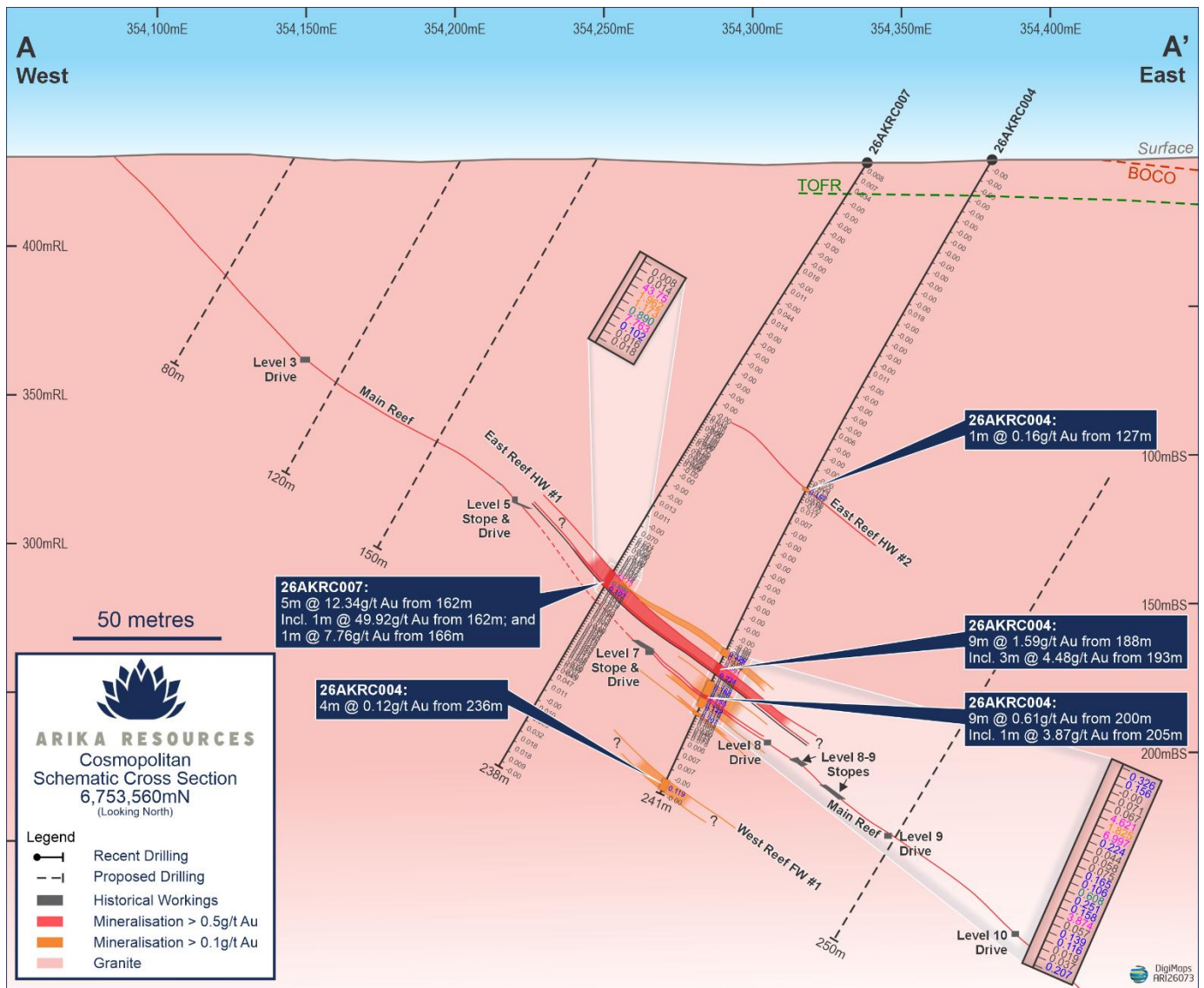
Figure 3: Schematic Cross-Section 6,753,560mN showing latest drilling results in relation to historical Level Drives and Stopes. Note: Holes 26AKRC004 and 26AKRC007 both intersected wide, high-grade gold mineralisation within a hangingwall position above the plane of historical mine development. Relatively weak mineralisation within what was interpreted by the underground miners to be the 'Main lode' may explain why no significant stoping was carried out within this area of the Cosmopolitan mine. Historical records report that hangingwall and footwall lodes to the 'Main Reef' were mined within the upper levels of the central part of the deposit but not to the north and south along strike nor at depth. The recognition of a strongly mineralised hangingwall structure well beyond the main historical workings presents an opportunity to outline significant ounces within extensive areas of the Cosmopolitan system which remain under-explored.
