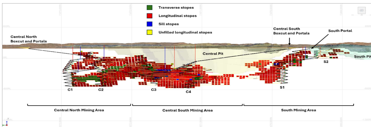
Figure 2 - Underground Ore Reserve Design (Long Section)
