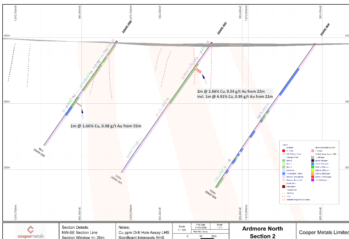
Figure 5 Ardmore North Section 2. 26MIE-004, 26MIE-005 and 26MIE-006.
