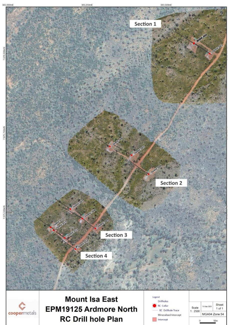
Figure 3 Ardmore North Drill Plan
