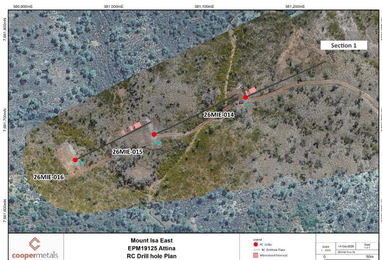
Figure 1 Attina drill plan
