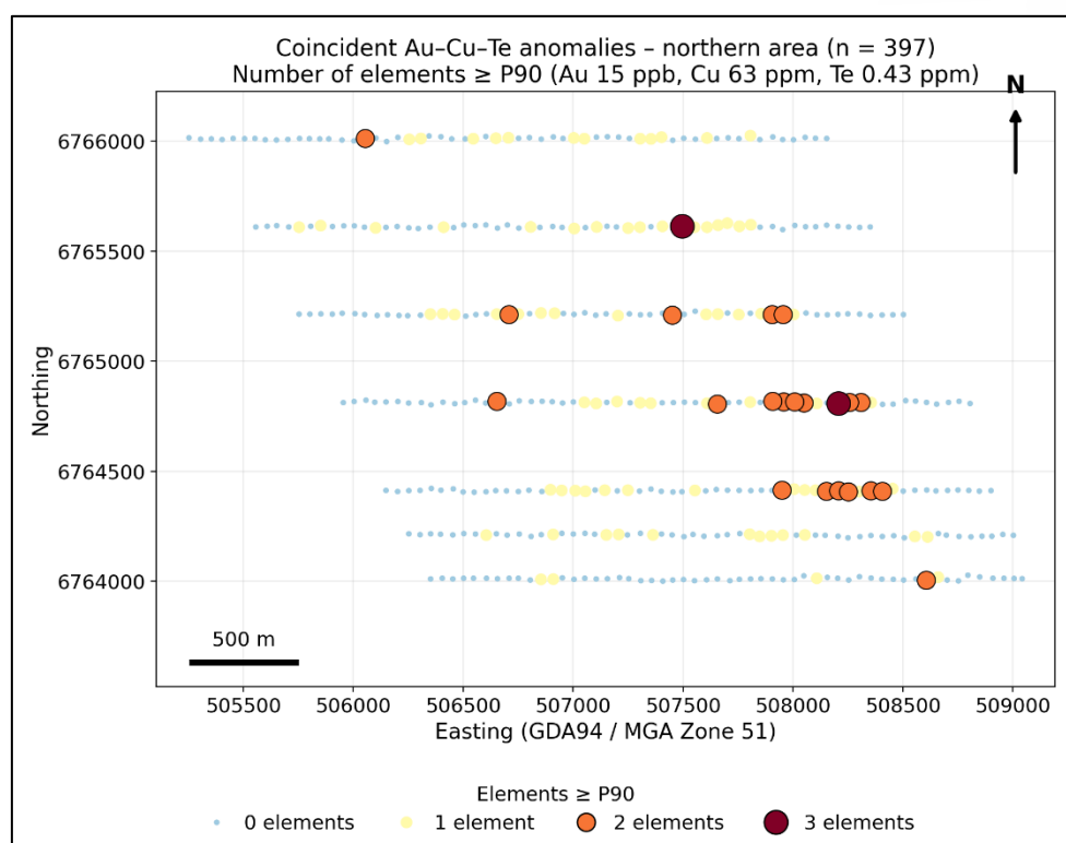
Figure 3 Stella Range Project, northern area. Number of elements (Au, Cu, Te) at or above the 90th percentile of the northern auger sample population (Au \geq 15 ppb, Cu \geq 63 ppm, Te \geq 0.43 ppm) in each sample (n = 397). Anomalous responses for all three elements are concentrated in the eastern part of the northern area, between approximately 507,600 mE and 508,400 mE.
