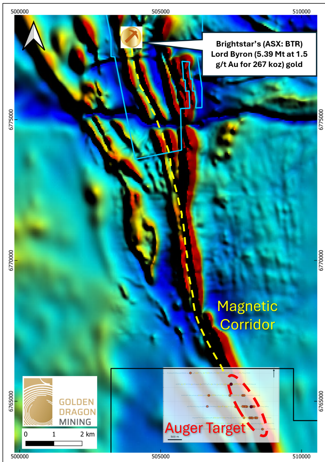
Figure 4 Coherent Au–Cu–Te cluster is interpreted to lie on the same north-north-west trending magnetic corridor as the Lord Byron gold deposit, approximately 12 km along strike
