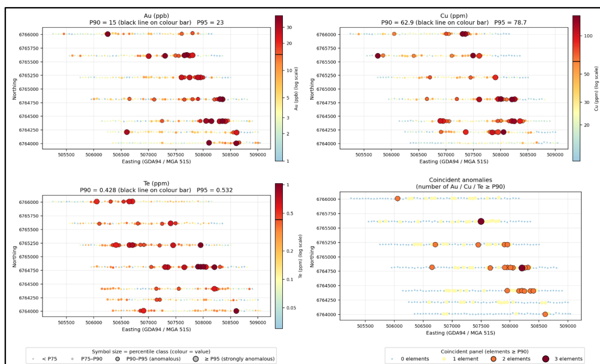
Figure 2. Stella Range Project, northern area. Auger geochemical results for gold (ppb), copper (ppm) and tellurium (ppm), with a panel showing the number of elements anomalous in each sample ( n = 397 ). Samples are coloured by value on a logarithmic scale from light blue (low) to dark red (high), and symbol size increases with percentile class (below P75, P75–P90, P90–P95, \geq P95). Anomalous samples (outlined in black) are those at or above the 90th percentile of the northern population: Au \geq 15 ppb, Cu \geq 63 ppm, Te \geq 0.43 ppm.
