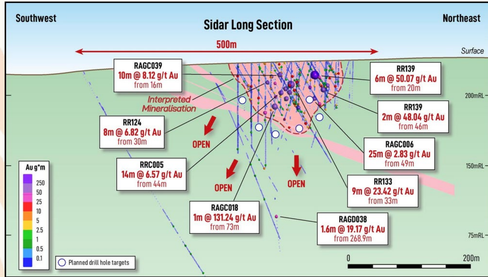
Sirdar Long Section showing gram metre pierce points, mineralisation interpretation outline (red) and pegmatite sill (pink), and planned RC drill targets.
