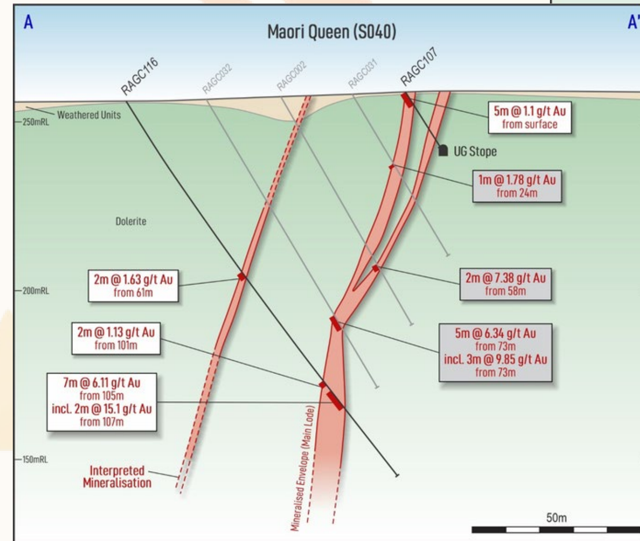
Cross section S040 showing drill intercepts, interpreted mineralisation and further down-dip potential
