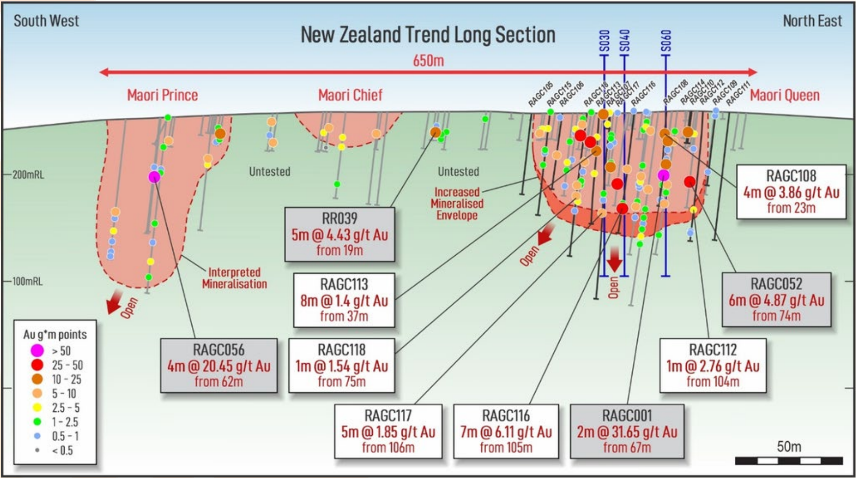
New Zealand Trend Long-section: Showing gram x metres intercepts, recent RC drilling and significant exploration potential
