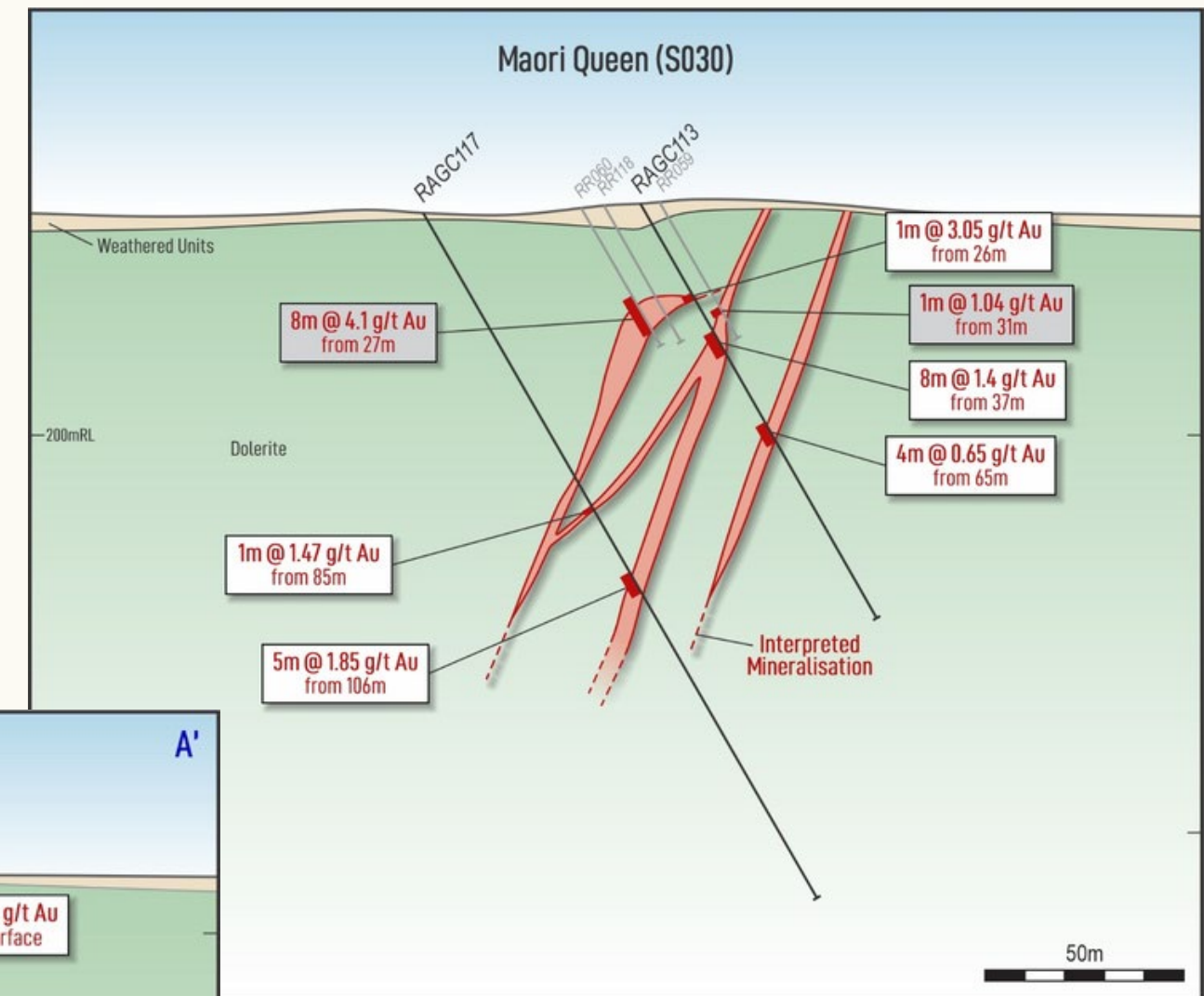
Cross-section S030 showing drill intercepts and down-dip potential
