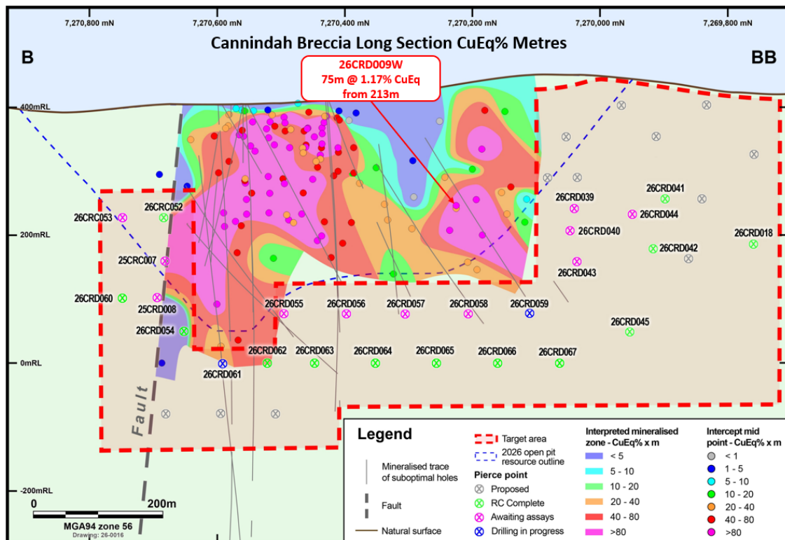
Figure 4: Cannindah Breccia Long Section showing location of 26CRD009W and current status of all drill holes
