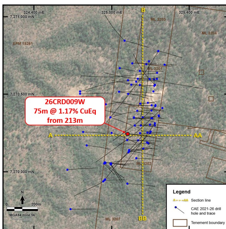
Figure 2: Location of drill hole 26CRD009W
