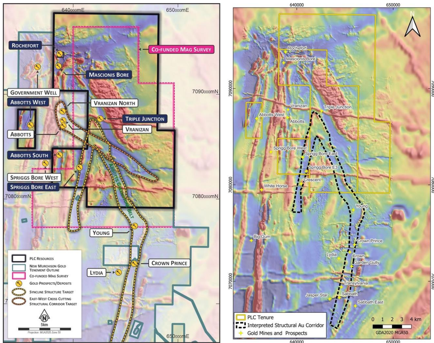
Figure 2: PLC's Abbotts Gold Project (outlined in black above left) sits about 35 km north of Meekatharra, in the northern part of the Abbotts Greenstone Belt. The magnetics map shows the interpreted syncline and cross-cutting structural corridor targets (left), and Abbotts interpreted structural corridor over magnetics (right). Neighbouring New Murchison Gold tenements and deposits shown for context only and are not PLC assets.
