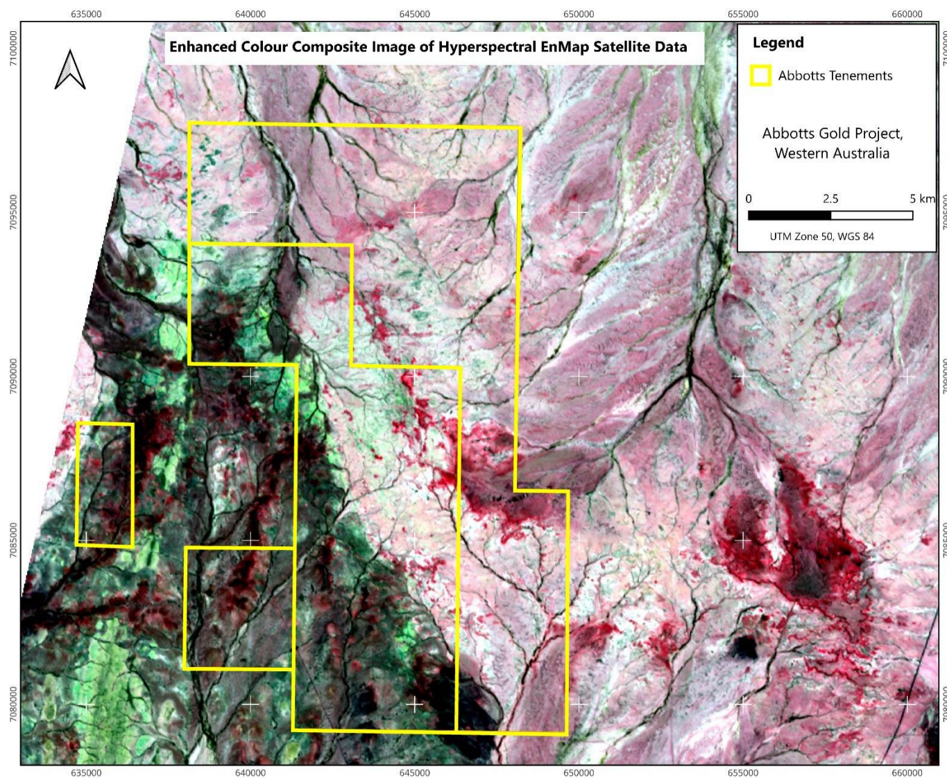
Figure 1: Hyperspectral EnMAP imagery over the Abbots Gold Project (224 spectral bands, 30 m resolution); Source: Geo Spectra Pty Ltd 3
