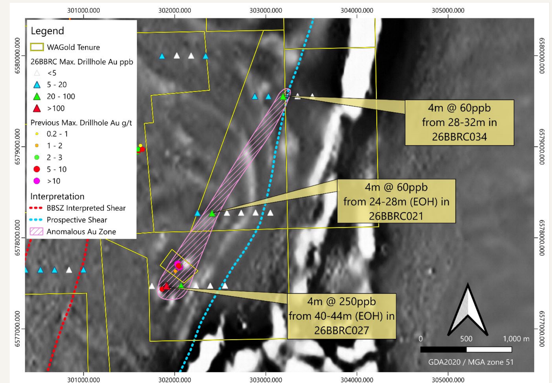
Bullabulling North: 2026 RC traverses over magnetic imagery
