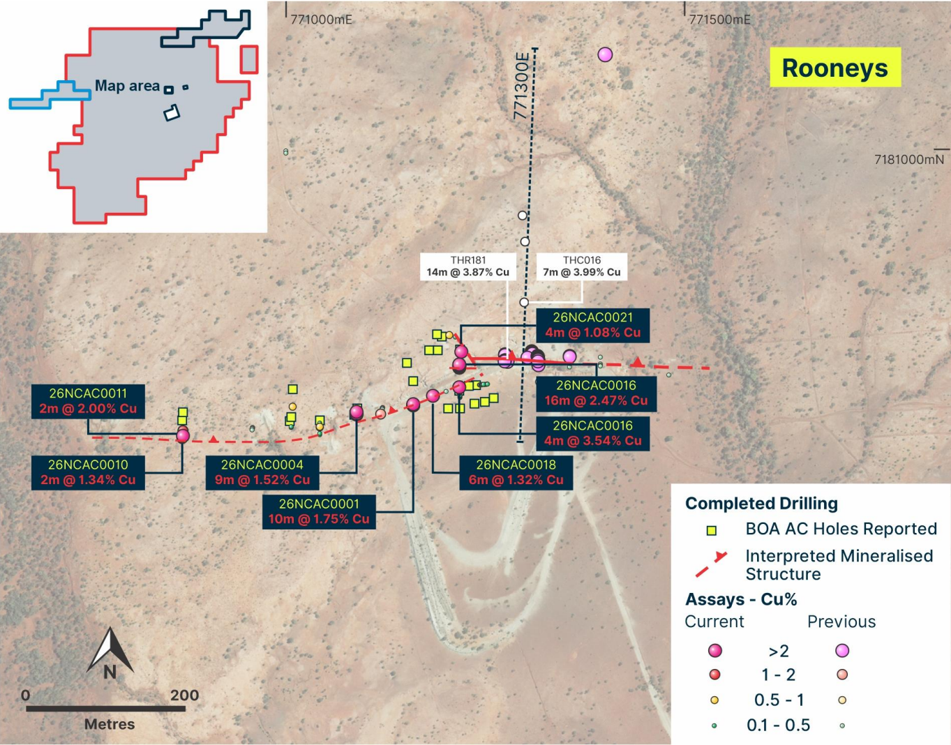
Figure 1: Rooneys drill plan showing drilling results and mineralised structures.
