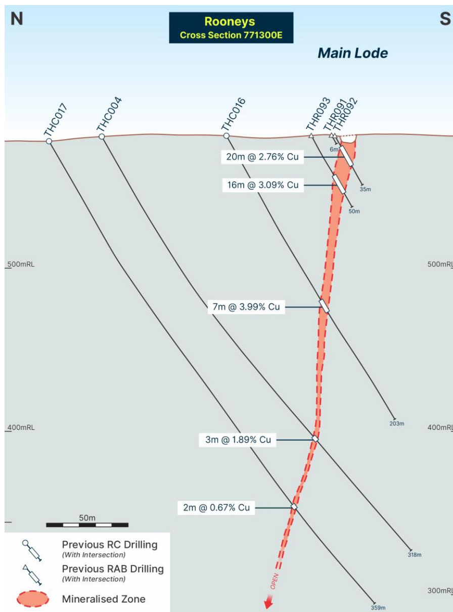
Figure 2: Rooney's Drill section 771300E
