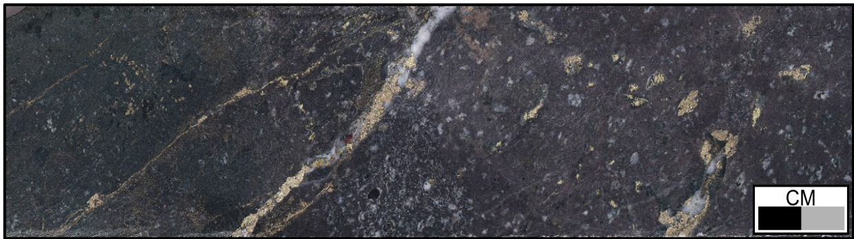
Figure 5: SPD083A at 718.2 m, 1 m @ 7.49 g/t Au. Quartz-pyrite- Au vein in chlorite-albite altered andesite
