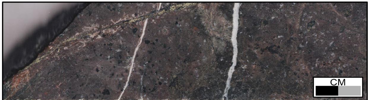
Figure 6: SPD083A at 715.5 m, 1 m @ 17.99 g/t Au. Chalcopyrite-quartz- Au vein in albite-chlorite altered andesite
