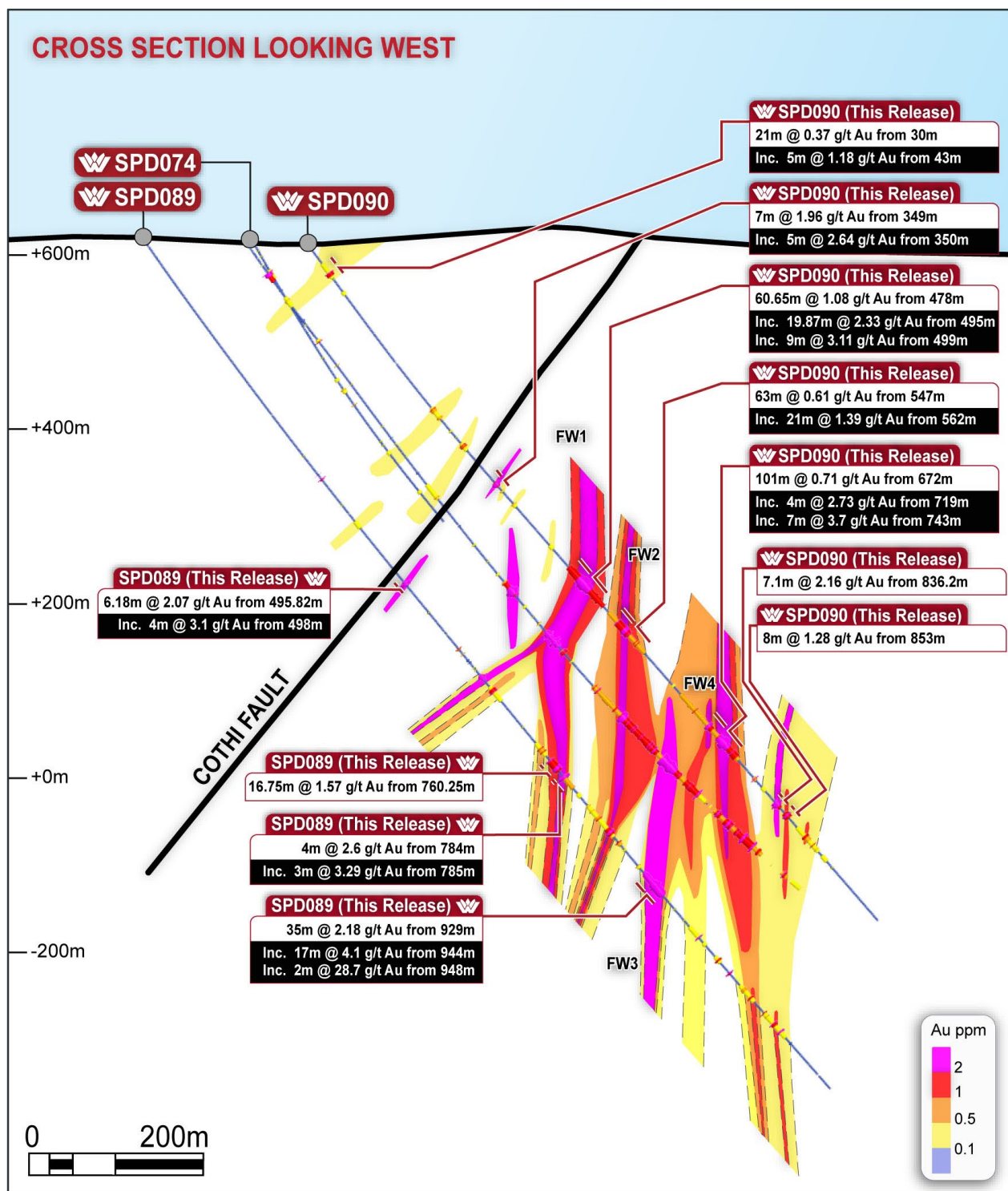
Figure 3: Spurr Project, Consols, section showing SPD090, SPD074 and SPD089. Looking West.
