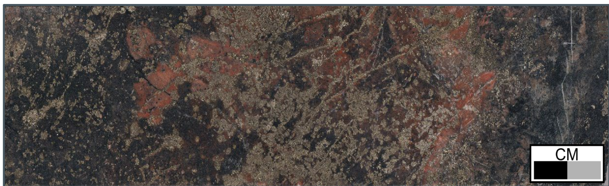
Figure 9: SPD082 at 566.8 m, 1 m @ 12.51 g/t Au. Strong pyrite disseminations and veining in a potassic altered andesitic autobreccia.
