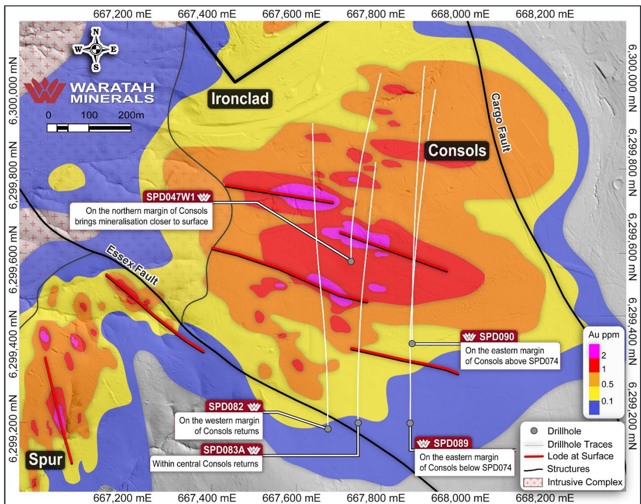
Figure 4: Consols Prospect, Spur Project, showing reported drilling results and growth potential. Gold mineralisation contours projected to surface.
