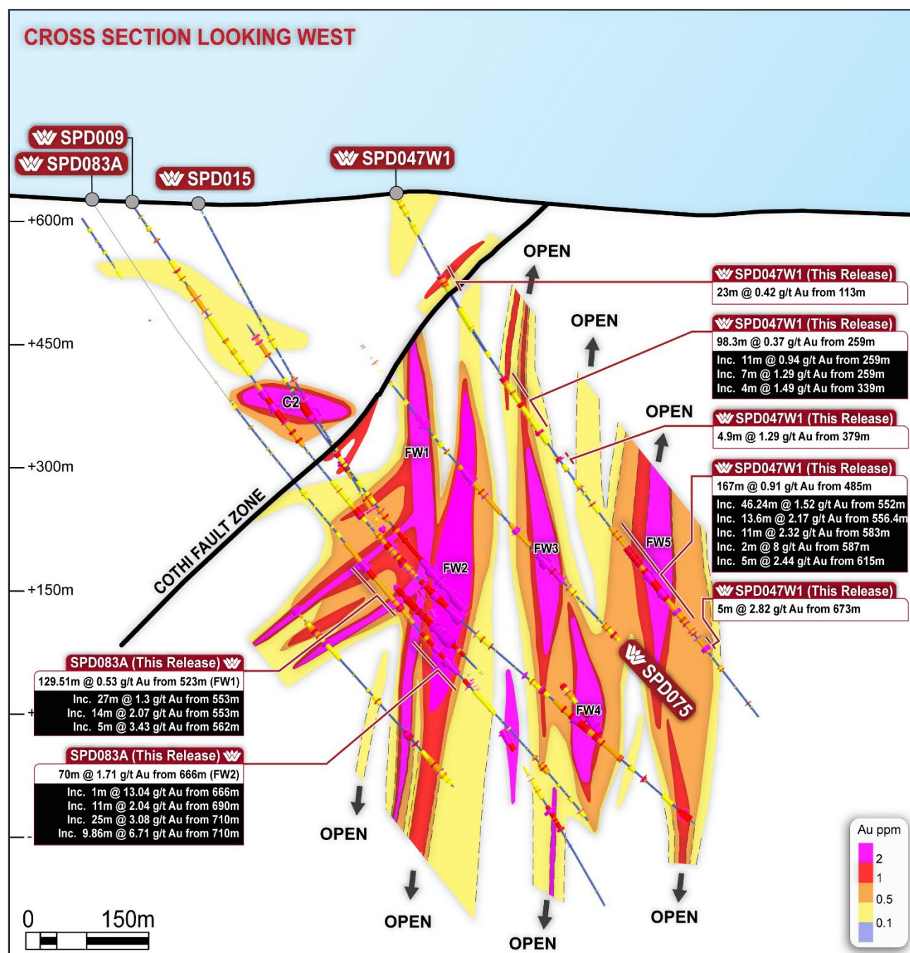
Figure 2: Spur Project, Consols, section showing SPD047W1, SPD083A and SPD009. Looking West.
