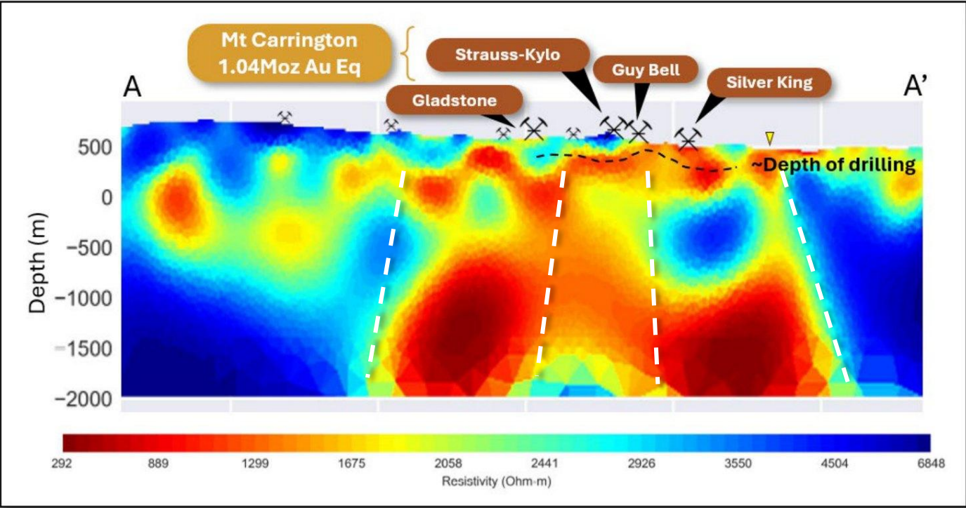
Airborne Mobile-MT conductivity section through the Mt Carrington group, historic workings and new areas of interest (LGM 2025).
