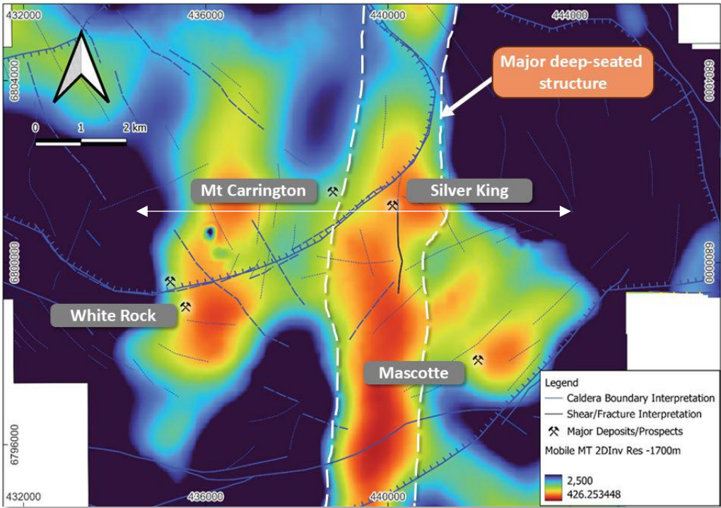
Airborne Mobile-MT conductivity plan view over the Mt Carrington central area (LGM 2025).
