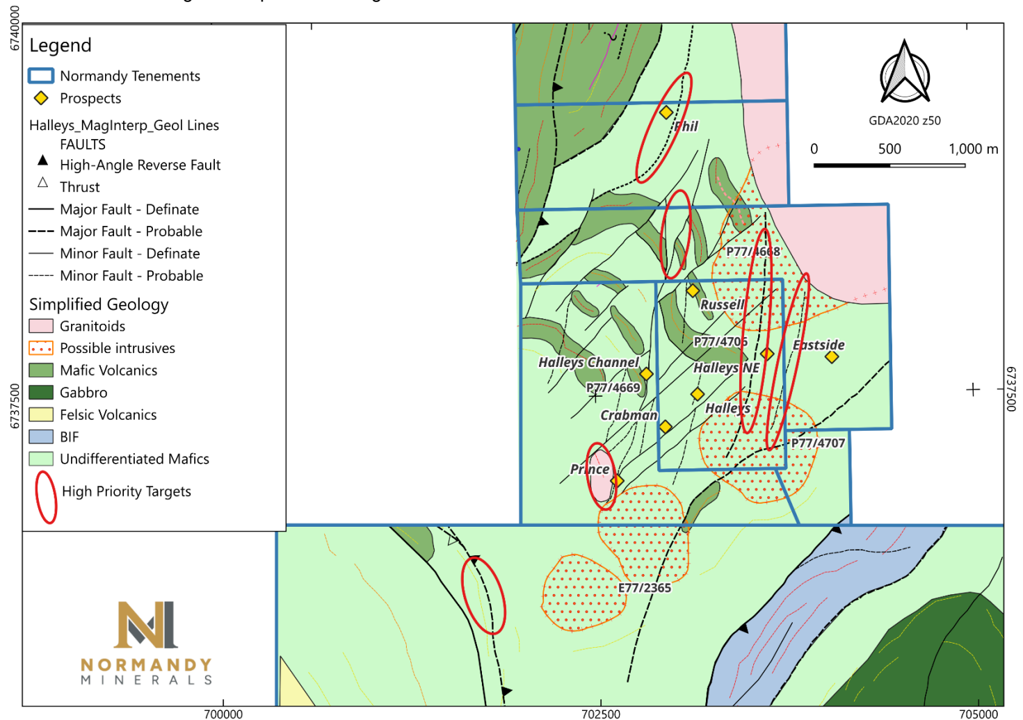
Figure 5: Halleys District geophysical interpreted geology and structural lines – showing interpreted northeast and north-northeast structures and possible intrusive bodies (Core Geophysics, 2026).
