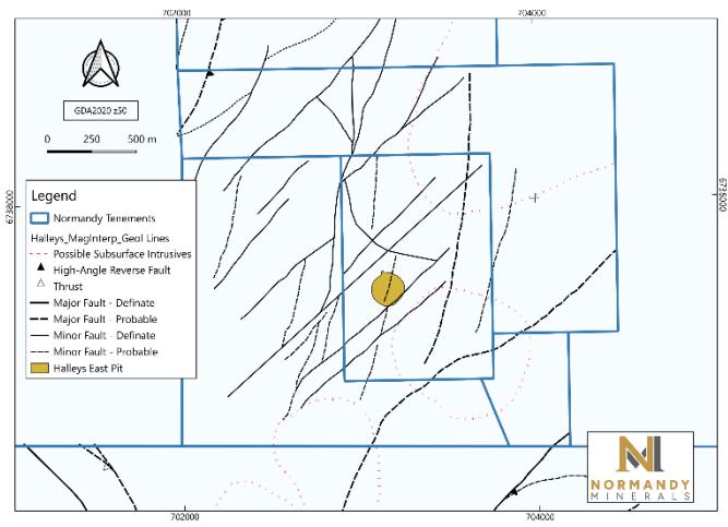
Figure 4: Updated Geological interpretation from Review.
