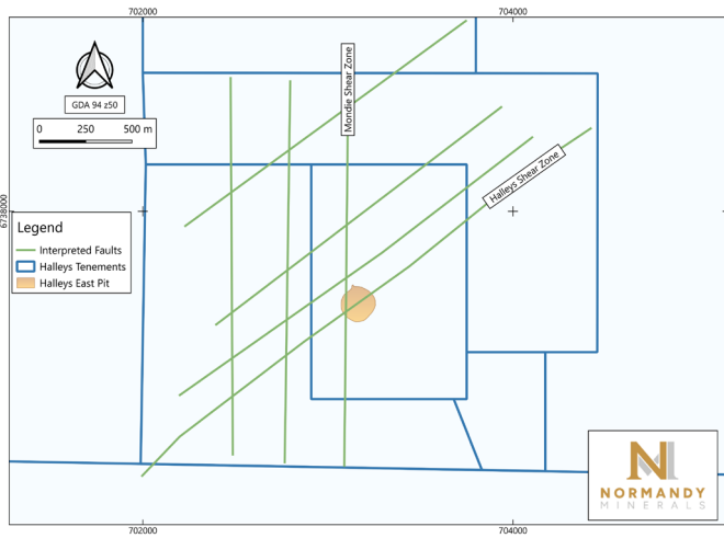
Figure 3: Previous Schematic representation of shallow drilling interpreted structures around Halleys Pit 1
