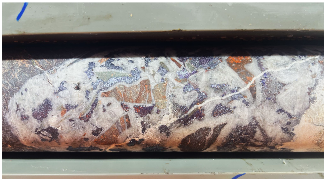
Figure 04 - Photograph of quartz-carbonate veining/brecciation hosting chalcocite-bornite mineralisation between logging interval 136.5-147.0m downhole in drill hole DAN26055. Core is NQ2 diameter.
