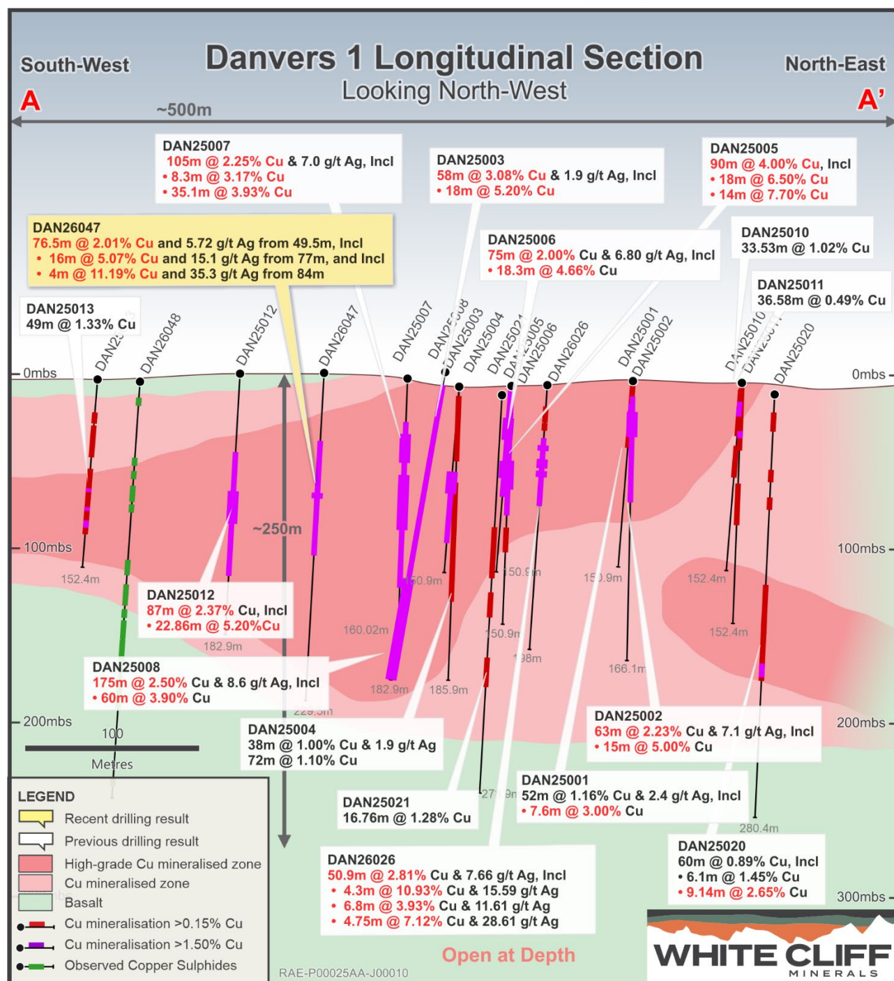
Figure 06 – Danvers 1 longitudinal section showing recently released DAN26047 which returned 76.5m @ 2.01% Cu from 49.5m and observations of copper sulphides from DAN26048, extending mineralisation to depth below previous drilling efforts. See ASX announcement dated 6 October 2026 “76.5m @ 2.01% Cu Expands Copper Envelope at Danvers 1”.
