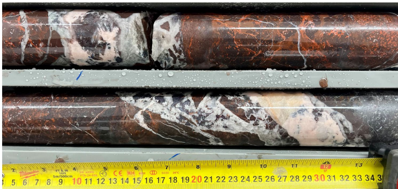
Figure 03 - Photograph of quartz-carbonate veining hosting chalcocite-bornite mineralisation between logging interval 136.5-147.0m downhole in drill hole DAN26055. Core is NQ2 diameter.
