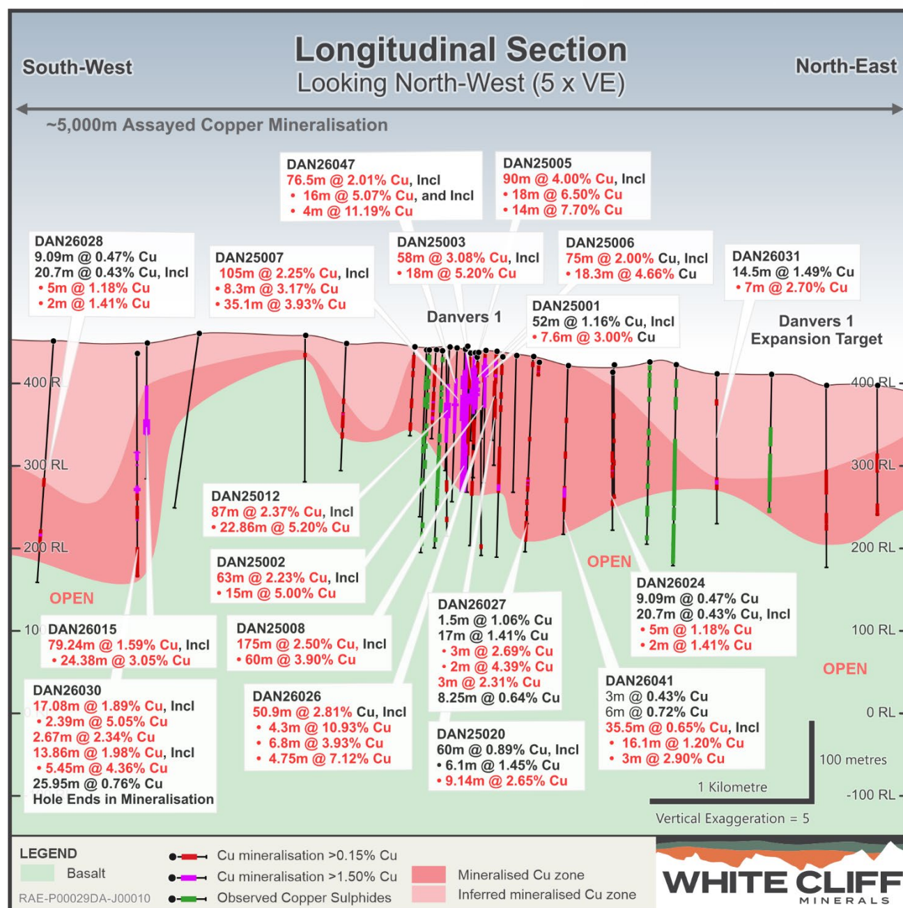
Figure 07 - Longitudinal section through the Danvers 1 deposit and extensions to the southwest and northeast. Reported drillholes DAN26051, 055, 057 have all returned intervals of copper sulphides to the northeast which can be seen as the green bars downhole. Green bars in Danvers 1 core zone represent pending assays from DAN26048, 049, 050 which targeted pinch points in the mineralisation model and all returned significant intervals of copper sulphides below existing mineralisation.
