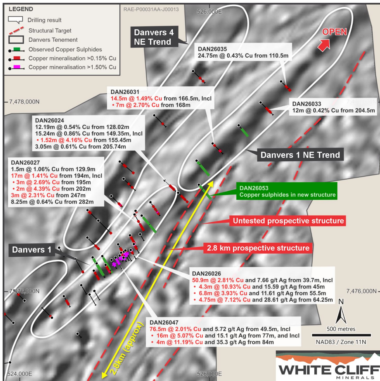
Figure 09 - Plan map of 2025 airborne magnetics (TMI RTP 1VD greyscale) depicting the clear NE magnetic low trend of Danvers 1 and Danvers 1 NE, and the Danvers 4 trend to the north. Highlighted by dashed red lines and the yellow arrow are a series of prospective structures that have not been drill tested apart from by DAN26053 which returned observations of copper sulphides within one of these structures. The structures are roughly parallel to the main Danvers trends.
