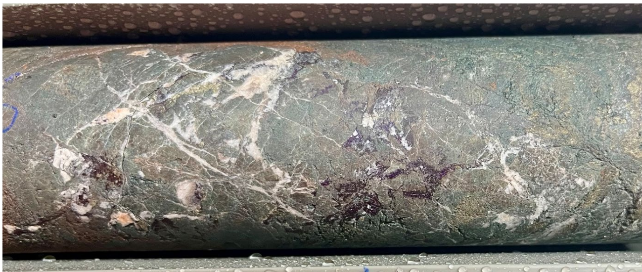
Figure 05 - Photograph of bornite-chalcopyrite-calcite cemented breccia from logging interval 165.65-183.6m downhole in DAN26055. Core is NQ2 diameter.
