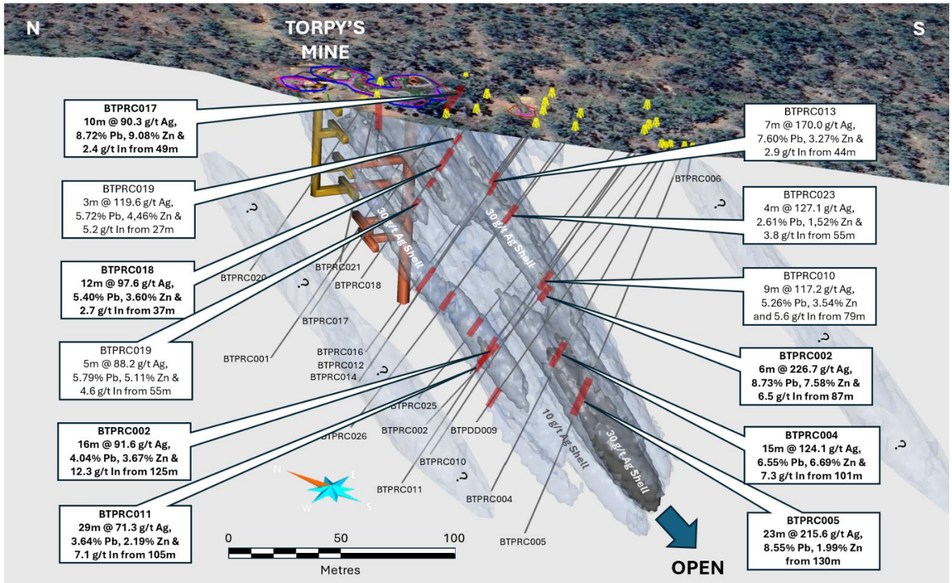
Figure 1 – Cross section of the Torpy's, looking northeast, showing significant drill results to date and modelled silver grade shells (i.e. 10 g/t and 30 g/t shells).
