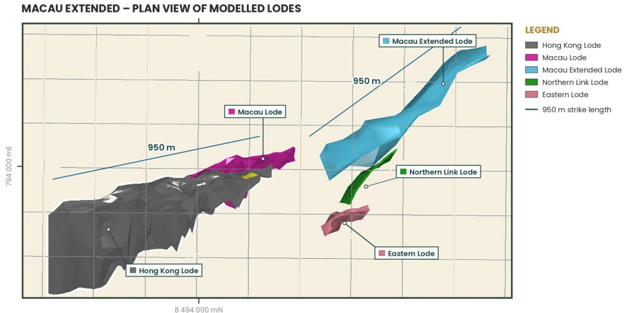
Figure 2: Plan view of ore lodes looking west showing Macau Extended, North Link and Eastern Lode extension
