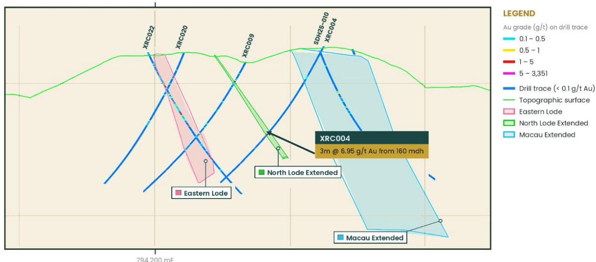
Figure 4: XRC004 intersected 3m @ 6.95 g/t Au from 160 mdh, some 50m away from the previously drilled SDH25-009
