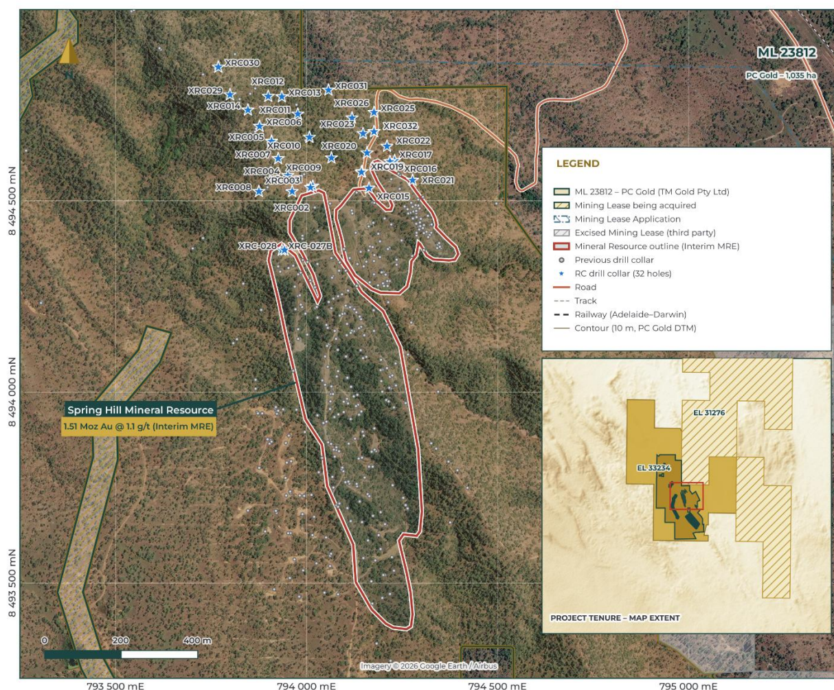
Figure 1: Spring Hill RC drill collar locations (32 holes drilled to date; assays reported for 22, with 10 pending), Mineral Resource outline (Interim MRE) and ML 23812 tenure
