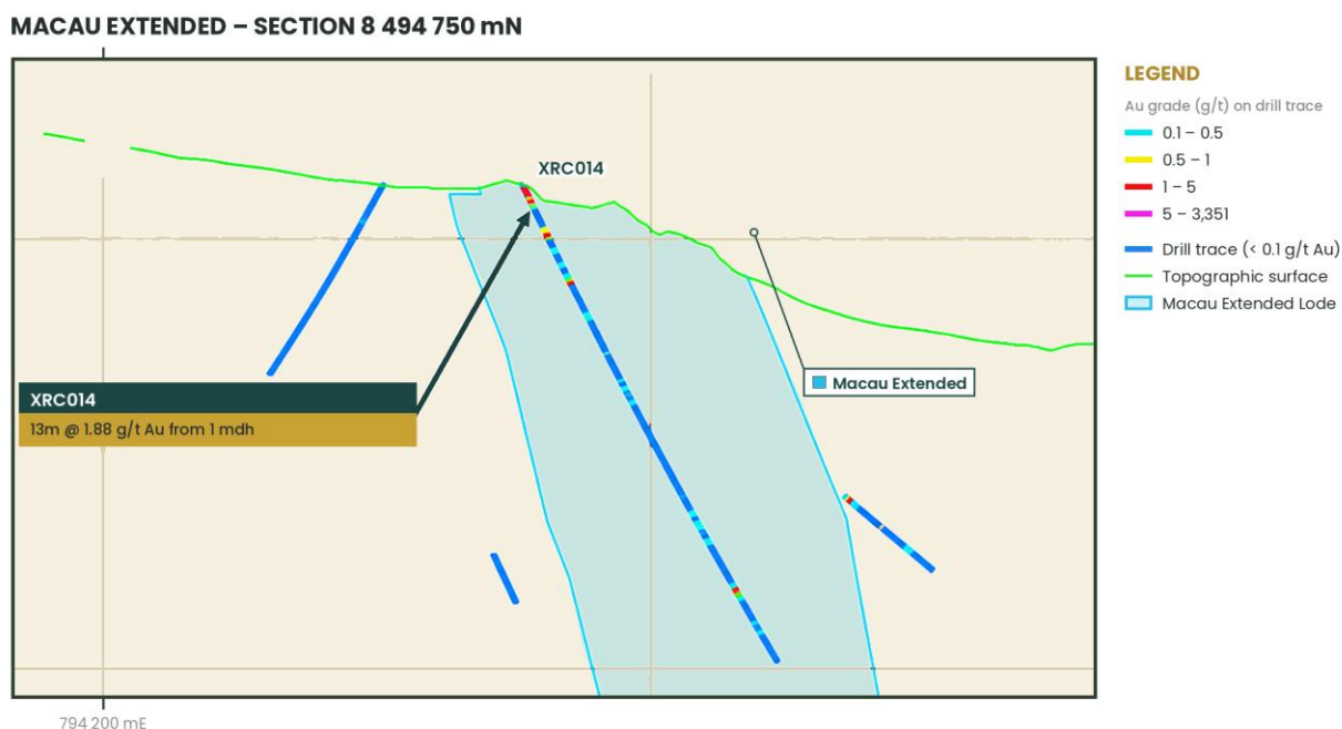
Figure 6: showing XRC014, 12m @ 1.88 g/t Au from 1 mdh
