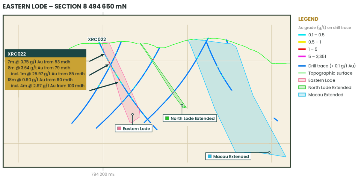
Figure 3: XRC022, multiple intercepts, including 8m @ 3.64 g/t Au in Eastern Lode mineralisation
