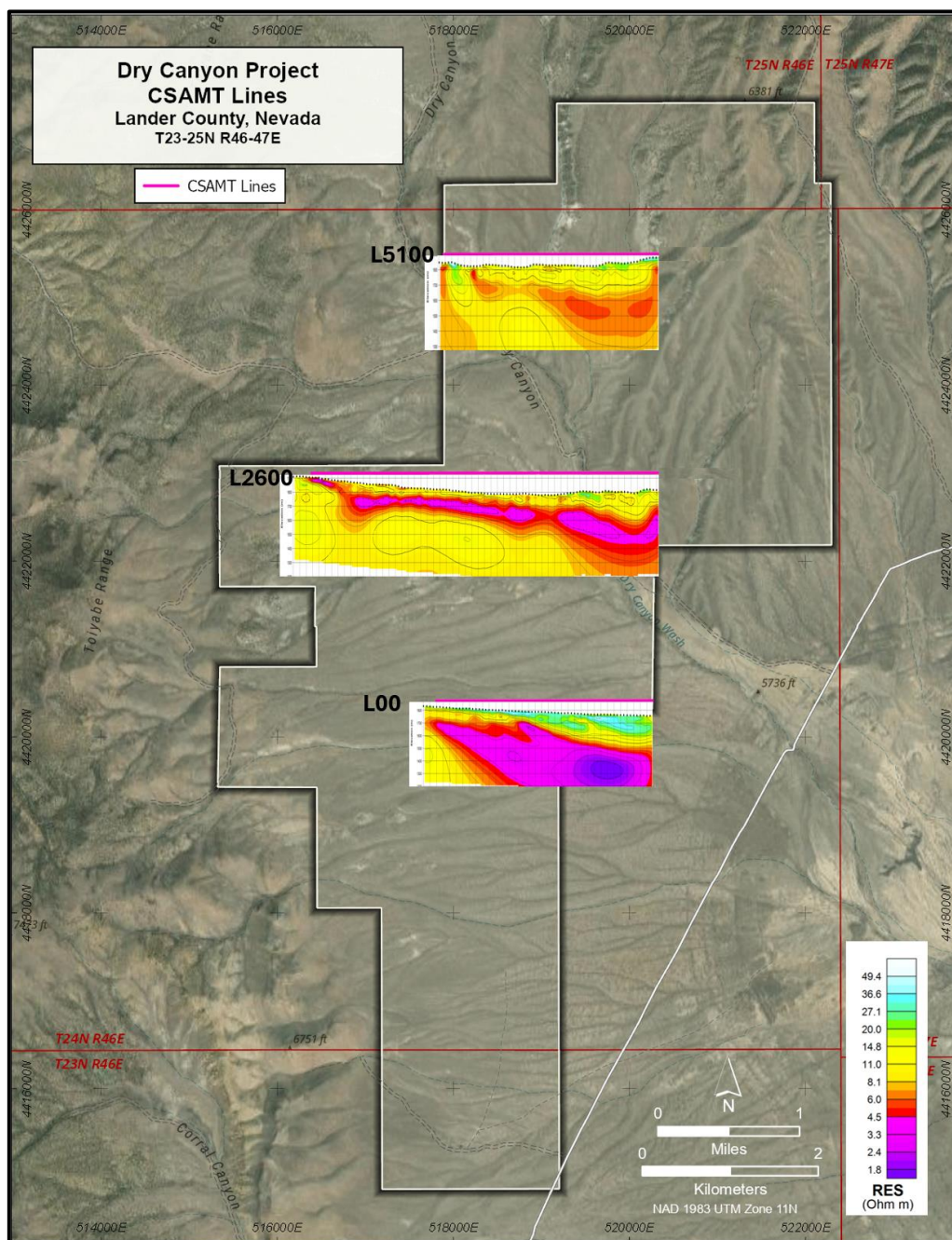
Figure 4. DRY CANYON CSAMT SURVEY 2D INVERSION RESULTS
