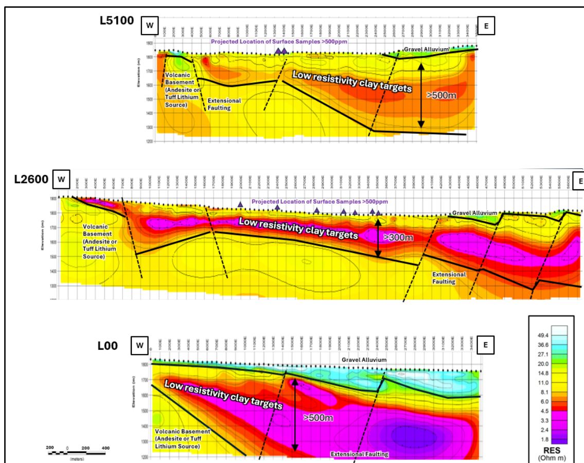
Figure 5. CSAMT 2D INVERSION DATA WITH BASIC INTERPRETATION
