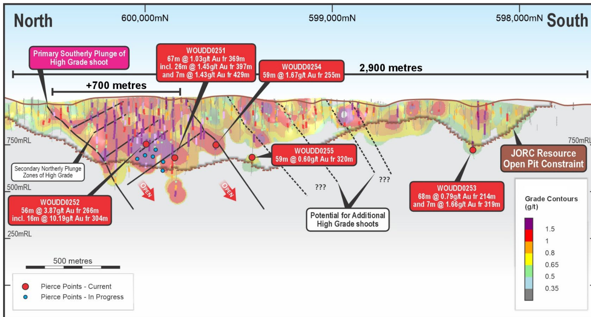
Figure Two | Woulo Woulo Long Section – Grade Contours
