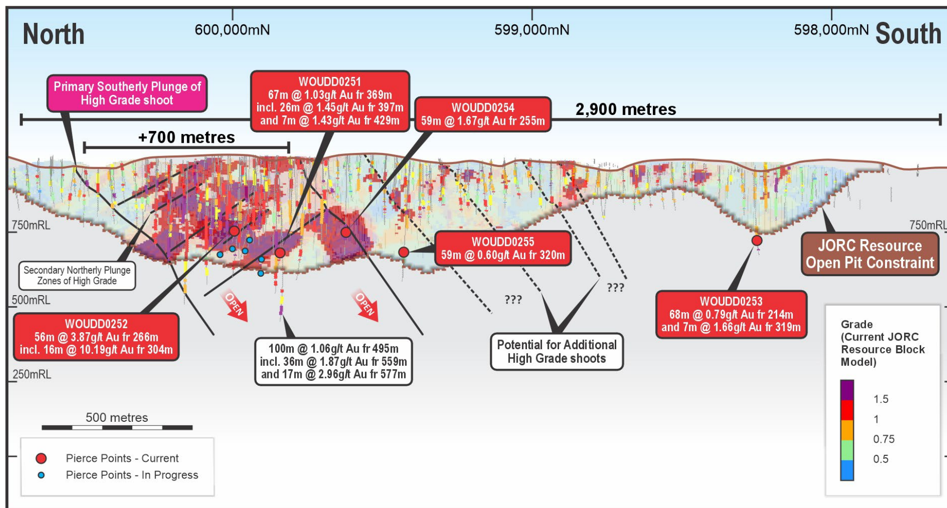
Figure Three | Woulo Woulo Long Section Block Model by Grade
