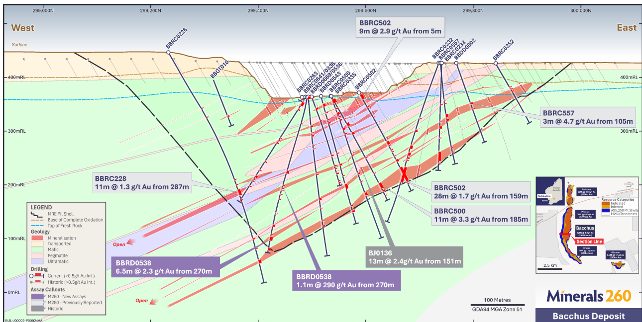
Figure 3: Section 6566330N showing mineralisation in BBRD0538 infilling Bacchus MRE pit shell (new results in purple boxes)
