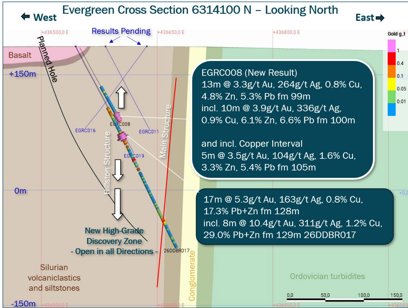
Figure 3: Cross section through the mineralised section in EGRC008 and 26DDBR017. (50m section).
