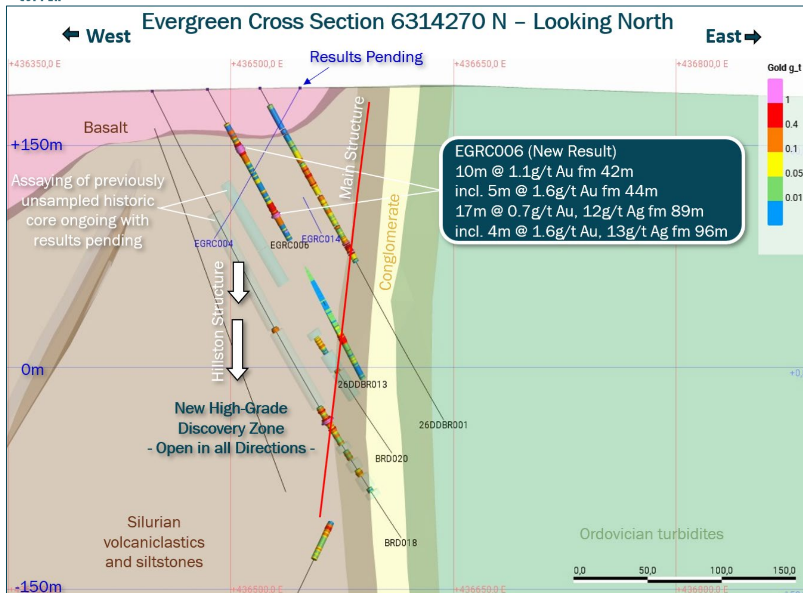
Figure 5: Cross section through the broad mineralised section in EGR006. (50m section).
