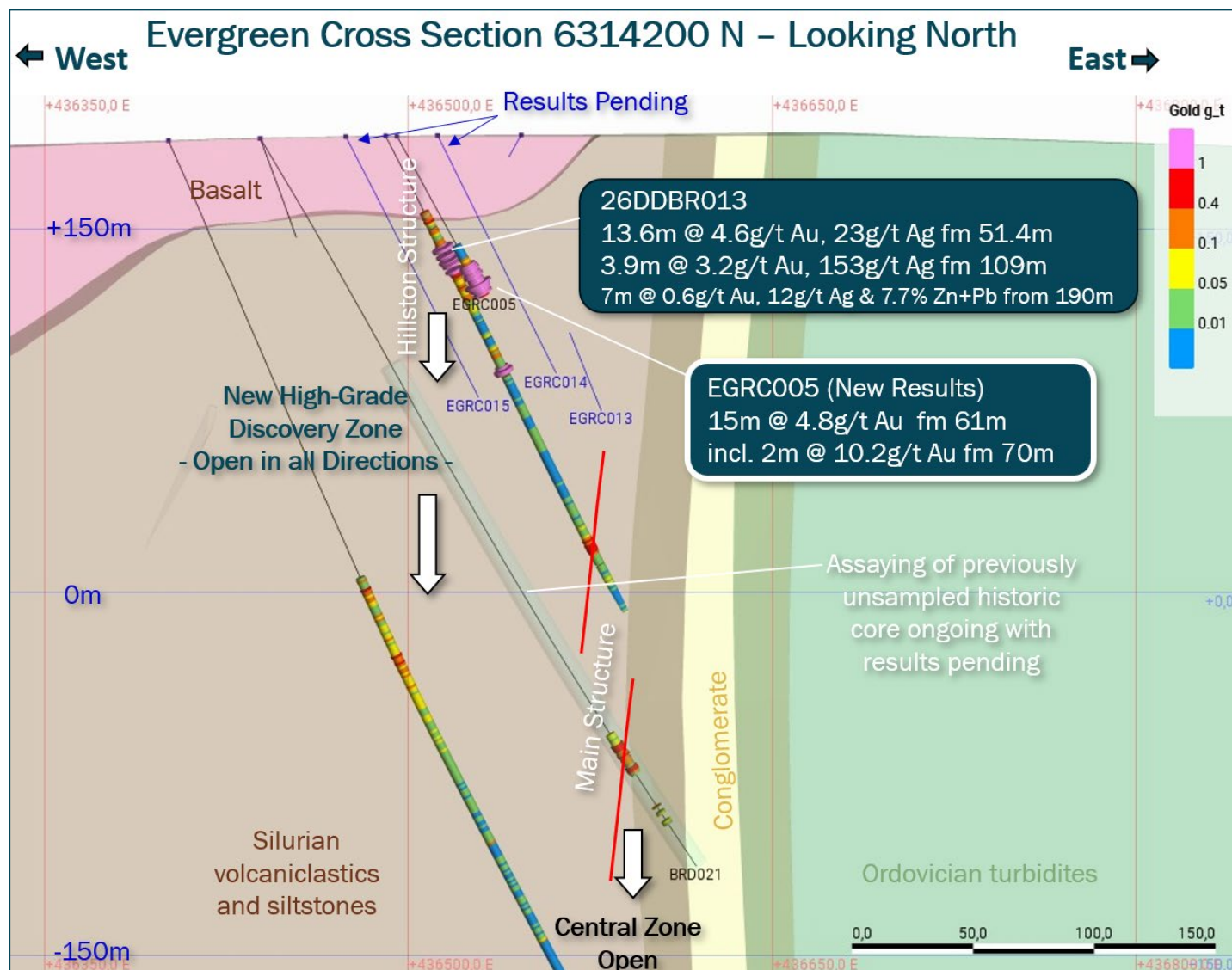
Figure 2: Cross section through broad mineralisation in EGRC005 and 26DDBR013. Holes with blue traces have assays pending. (50m section).
