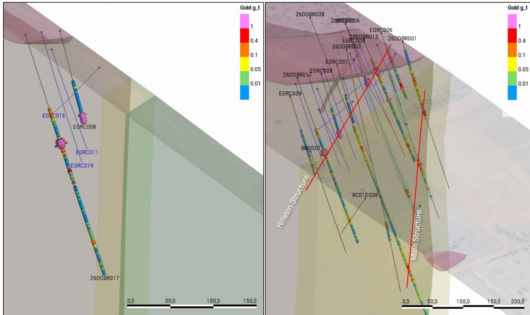
Figure 4: Oblique views looking down and to the north west at EGRC008 and 26DDBR017 with two holes pending assays 50m clipping (left) and 300m clipping showing results and holes with assays pending in blue traces (right).
