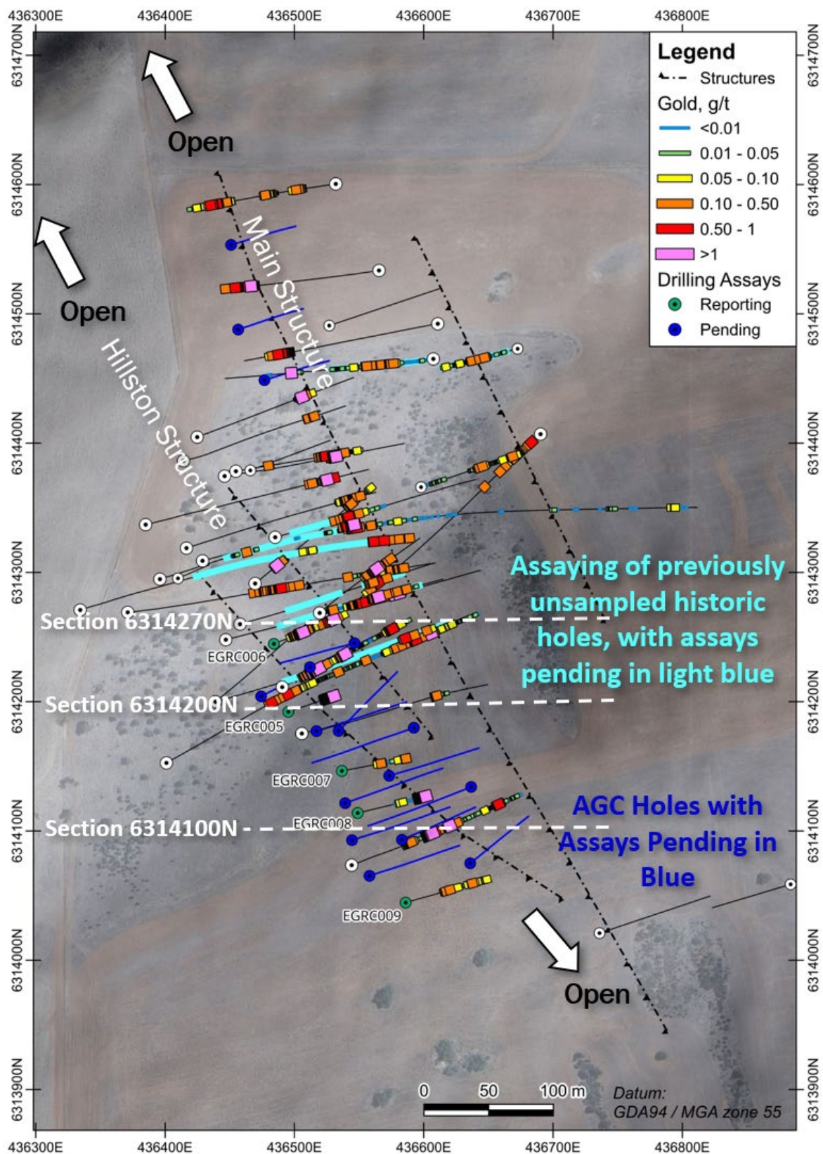
Figure 6: Plan map showing gold results at Evergreen with holes being reported with green collars, holes pending assays with blue collars.
