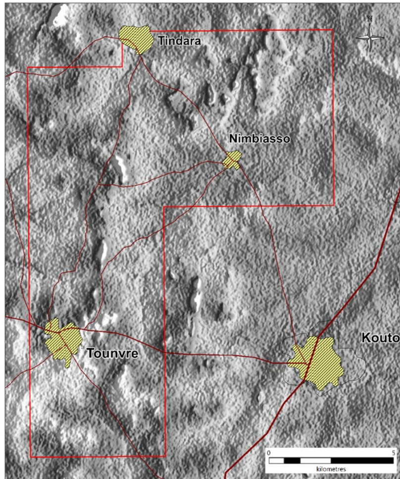
Figure 5: Map showing the boundary of the Atex lithium project tenement area (PR0777) in red and key villages and towns with road access in brown. Background is greyscale DEM from historical regional geophysical survey.
