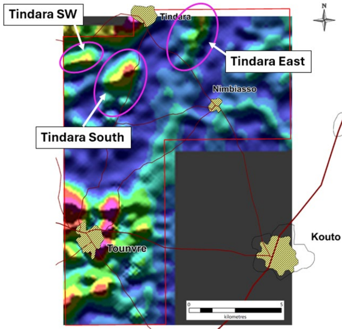
Figure 3: Map of the Atex lithium project showing the distribution of Rb in soil with priority auger drilling and/or trenching targets outlined in pink. Tindara South and to a lesser degree Tindara SW also display coincident pronounced Li and Nb anomalism in soil (refer ASX Announcement dated 7 September 2026).
