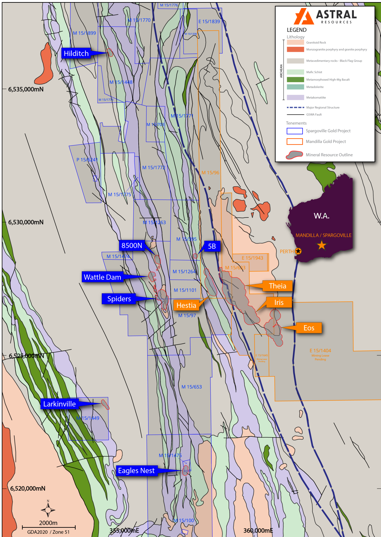
Figure 5 – Map of Spargoville and Mandilla Gold Projects on local area geology.
