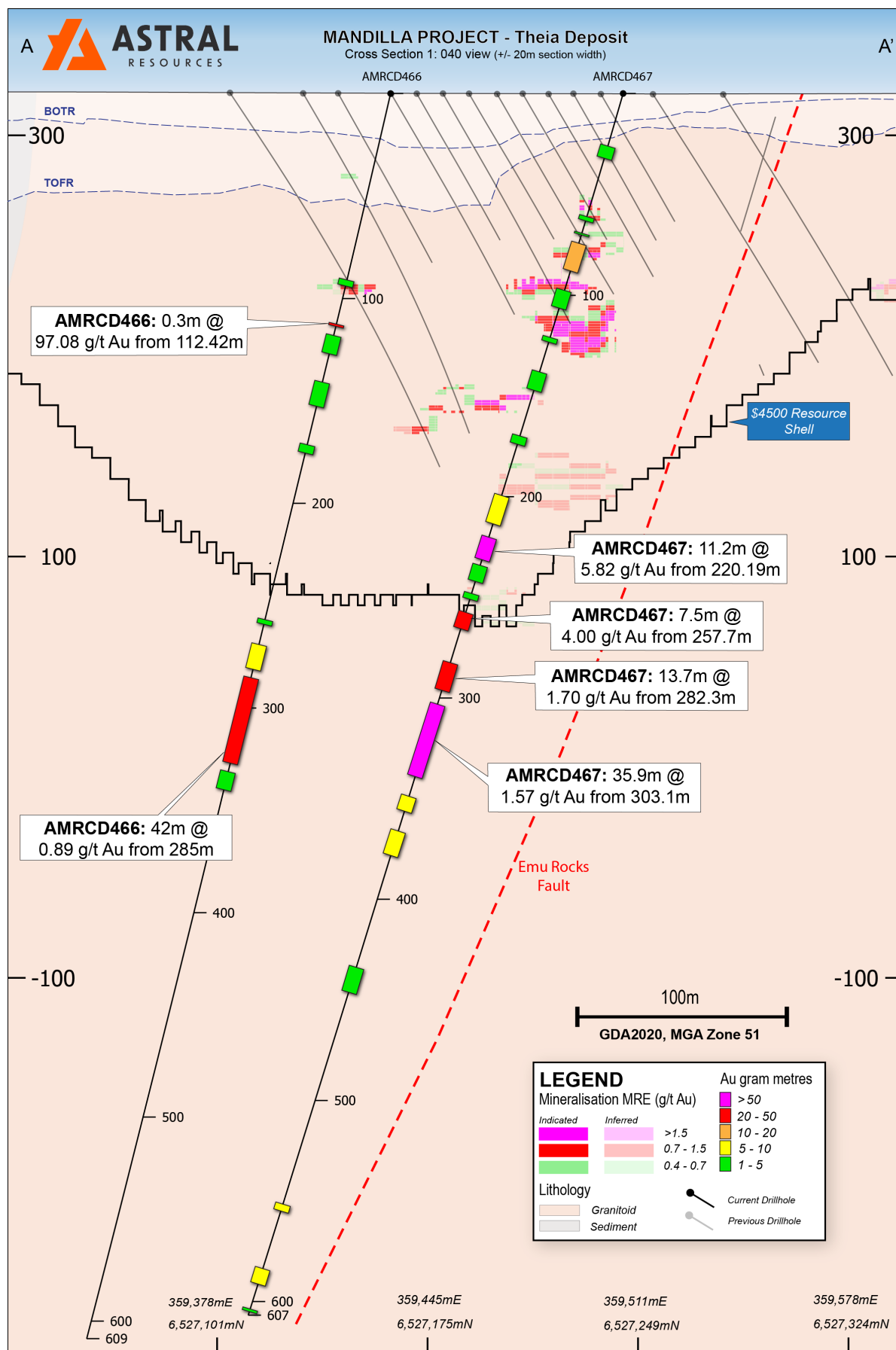
Figure 4 – Cross-section view of the Theia Deposit showing AMRCD466 and AMRCD467
