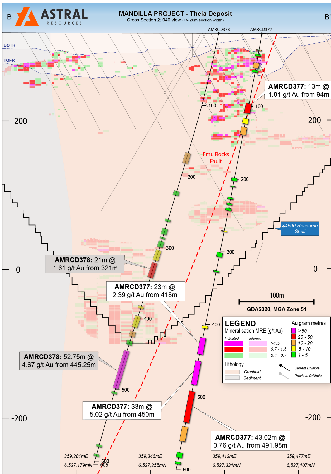
Figure 3 – Cross-section view of the Theia Deposit showing AMRCD377 and AMRCD378.
