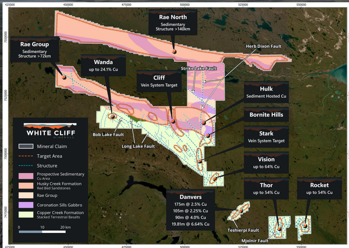
Rae District Sedimentary Targets
