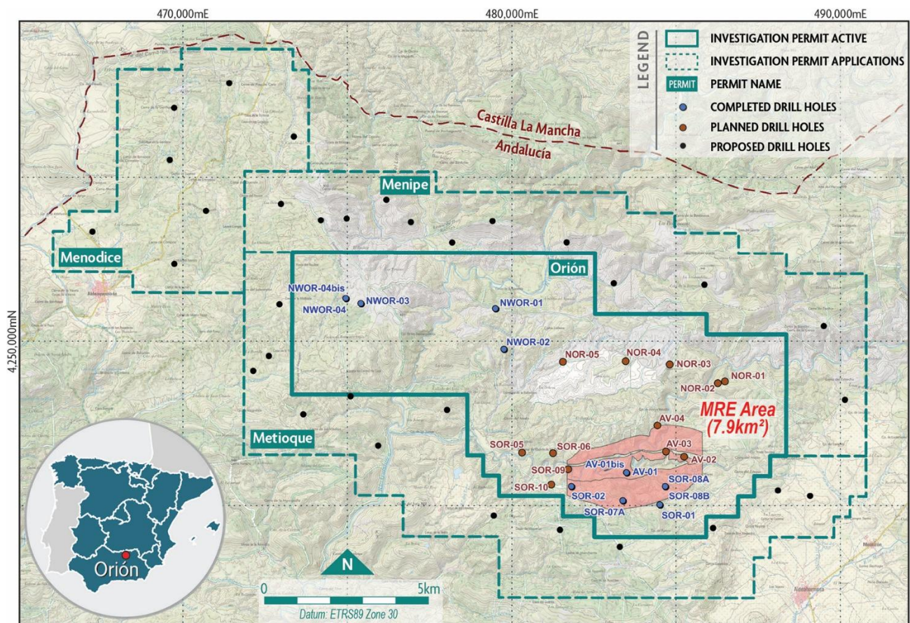
Figure 1 – Map Showing Orión Project Area with Planned Drill Holes in Maroon. Blue samples denote completed holes, except SOR-08B, which is in progress.
