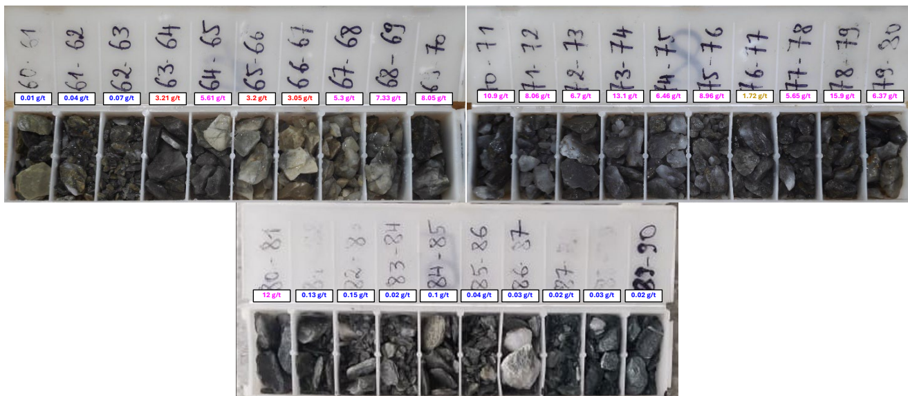
Figure 5. Close-up of the mineralised zone in BDR002 with grades associated with corresponding intervals (refer Reference 6).
