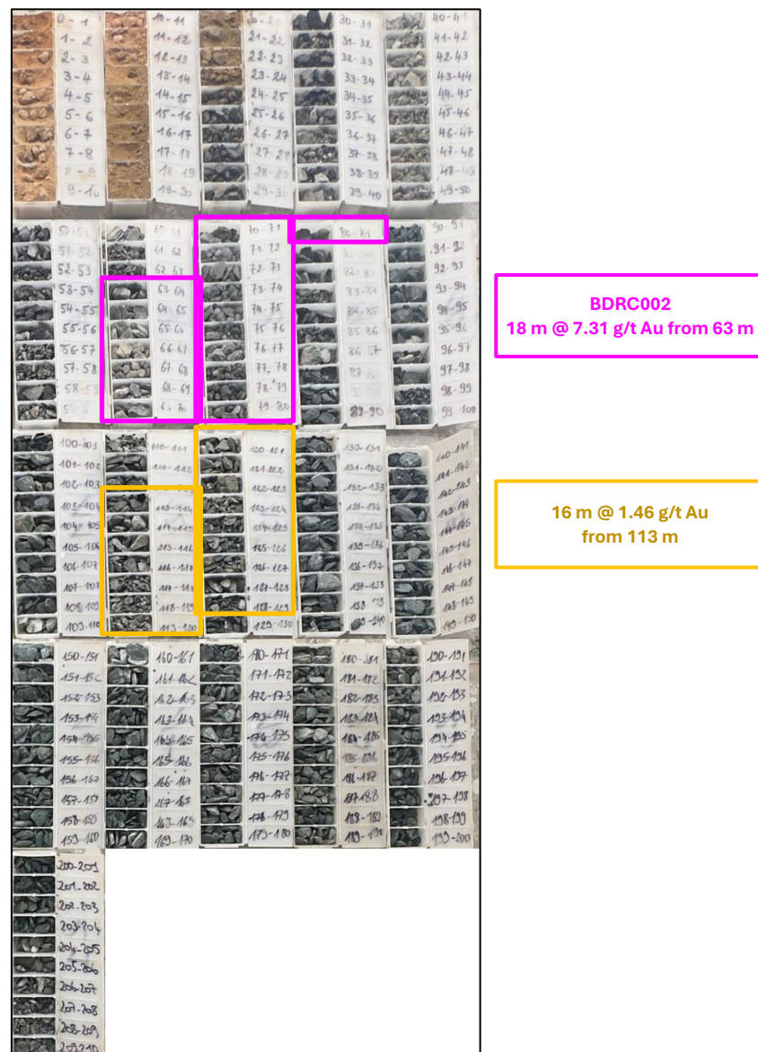
Figure 4. BDR002 chip trays showing previously reported assay intercepts (refer Reference 6).
