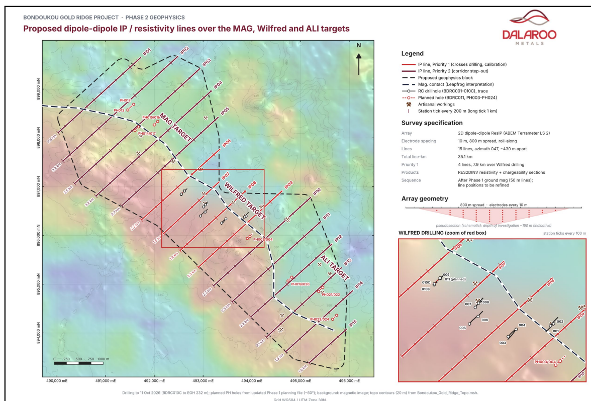
Figure 8. Proposed IP survey on magnetics: 15 lines (35.1 line-km) across magnetic contact. Priority 1 (red) crosses Wilfred; Priority 2 (maroon) extends to Mag and Ali.
